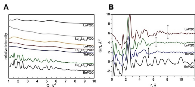
Figure 5. A) Powder X-ray diffraction data for \text{LnPQQ} species after background subtraction (P02.1 beamline at the PETRA III; \lambda = 0.20714 \text{ \AA} ; empty capillaries were used for background subtraction). B) Pair distribution functions for \text{EuPQQ} , \text{TbPQQ} , \text{LuPQQ} and \text{LaPQQ} species (vertical marks show qualitative cut offs in interatomic correlations for amorphous species).
