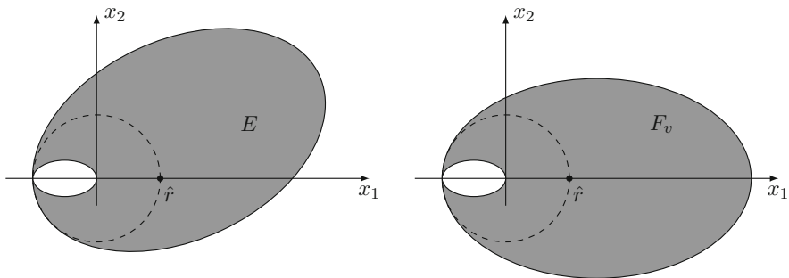
Fig. 3 The set E above cannot be obtained by applying an orthogonal transformation to the set F_v shown in the right, therefore rigidity ( \mathcal{R} ) fails. This happens because the set \{0 < \alpha_v < \pi\} is disconnected by a point \hat{r} \in (0, \infty) such that \alpha_v(\hat{r}) = \pi
