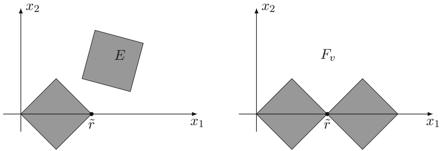
Fig. 2 Rigidity ( \mathcal{R} ) fails, since the set \{0 < \alpha_v < \pi\} is disconnected by a point \tilde{r} \in (0, \infty) such that \alpha_v(\tilde{r}) = 0
