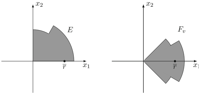
Fig. 5 An example in which rigidity fails. In this case, the tangential part of \partial^* F_v gives a non trivial contribution to P(F_v) . This allows to slide a proper subset of F_v around the origin, without modifying the perimeter
