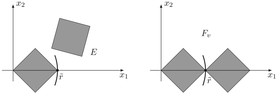
Fig. 4 Modifying the function \alpha_v given in Fig. 2 at the point \tilde{r} , we can make sure that \{0 < \alpha_v < \pi\} is an open connected interval. However, rigidity still fails
