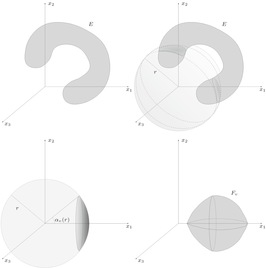
Fig. 1 A pictorial idea of the spherical symmetral F_v of a v -distributed set E , in the case n = 3
