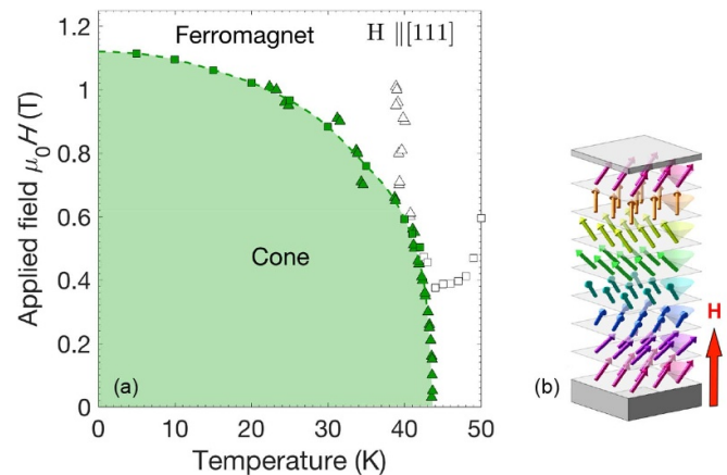
Figure 13. (a) Magnetic phase diagram of a 25.4 \text{ nm} = 1.83L_D thick MnSi(111) film grown on Si(111) derived from magnetometry measurements. The magnetic field H is applied along the film normal. An illustration of the cone phase is shown in (b). Reprinted figure with permission from [135], Copyright (2014) by the American Physical Society.
