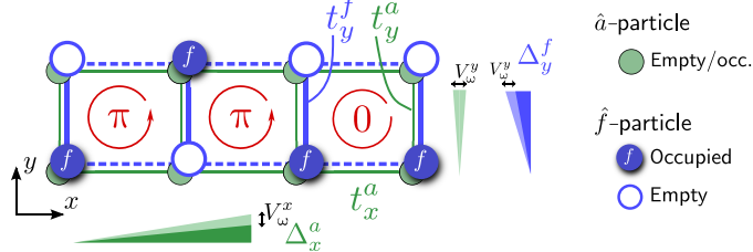
Fig. 5. Implementing matter-gauge field coupling in a two-leg ladder. Multiple double-well systems as described in Fig. 2 are combined to form a two-leg ladder by including hopping elements t_x^a of the a -particles along the x direction. Coherent tunneling is first suppressed by strong interspecies Hubbard interactions U and static potential gradients: \Delta_x^a = U for a -particles along x , and \Delta_y^f = U for f -particles along y . These gradients are indicated by triangles whose colors refer to the respective atomic species. The tunnel couplings are restored by a resonant lattice shaking with frequency \omega = U , realized by a modulated potential gradient V_\omega(\mathbf{j}, t) = (j_x V_\omega^x + j_y V_\omega^y) \cos(\omega t) seen by both species. The modulated gradients are indicated by light-colored triangles. We assume that each rung is occupied by exactly one f -particle, which can thus be described by a link variable, while the number N_a of a -particles is freely tunable. As shown in section S2, the special choice for the driving strengths V_\omega^a/\omega = V_\omega^f/\omega = x_{02} leads to an effective Hamiltonian with matter coupled to \mathbb{Z}_2 lattice gauge fields on the rungs. The gradient \Delta_x^a = U guarantees that the a -particles pick up only trivial phases \hat{\phi}^x = 0 while tunneling along the legs of the ladder. Hence, the Aharonov-Bohm phases (red) associated with the matter field become 0, or \pi corresponding to a vison excitation. They are determined by the plaquette terms \hat{B}_p defined in Eq. 20, reflecting the configuration of f -particles.
