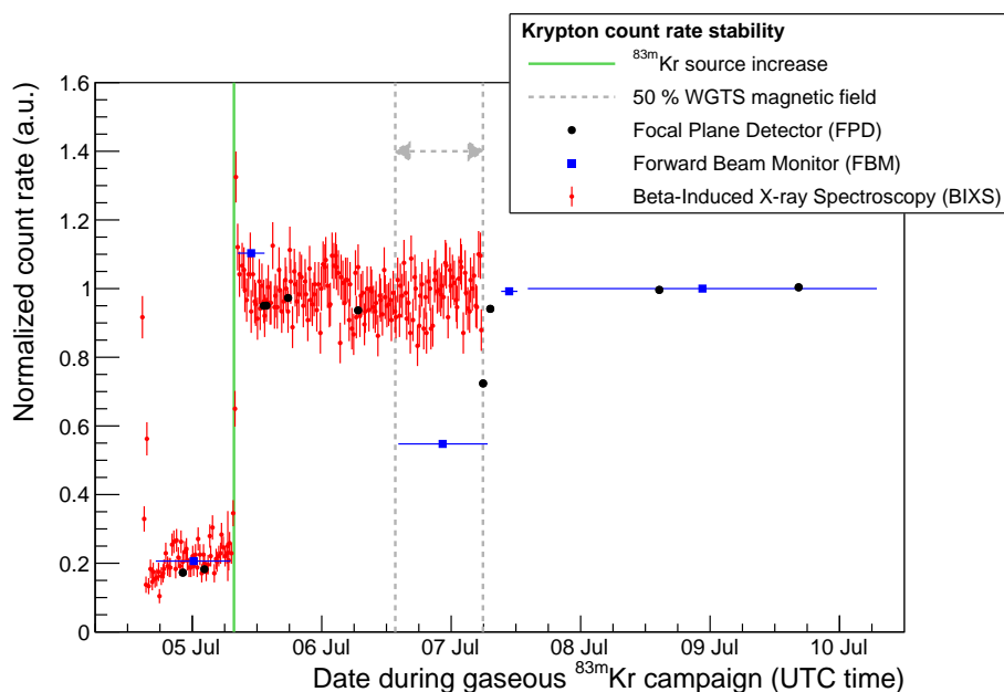
Figure 18. Normalized relative count rates from three KATRIN detector systems during the gaseous ^{83\text{m}}\text{Kr} campaign. FPD data, at a 0.27 mT setting, are shown in black circles; FBM data are shown in blue squares; and BIXS data are shown in red dots. The data from all three detectors are normalized to one in their respective stable regions. Vertical lines indicate hardware changes during the campaign. All three detectors observed approximately a fivefold increase in count rate when the ^{83\text{m}}\text{Kr} source intensity was increased (green line). The FPD and FBM observed a decrease in count rate (approximately 20 % and 50 %, respectively) when the WGTS had a lowered magnetic field (gray lines), while BIXS was insensitive to the WGTS magnetic field. Statistical errors in FPD and FBM data are too small to be visible. BIXS data-taking was stopped on 7 July.
