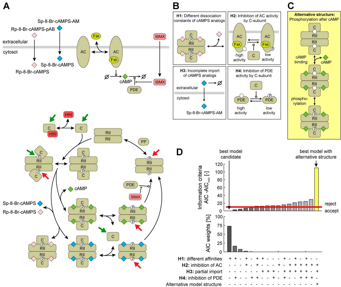
Figure 7. Mechanistic mathematical modeling supports that RII phosphorylation occurs before opening of PKA-II holoenzymes. (A) Illustration of the core PKA-II model. Colored arrows indicate accessible epitopes recognized by pRII (red) and Ca (green) antibodies, respectively. (B) Illustration of model extensions allowing for differences between cAMP analogues (H1 and H3) and feedback regulation (H2 and H4). (C) Illustration of an alternative model structure assuming that cAMP induces RII phosphorylation. (D) Ranking of model hypotheses according to the AIC value.
