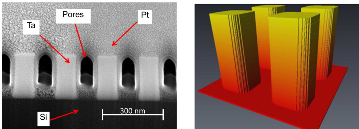
Figure 5.10: SEM image of Ta column cross-section (left) and 3-D model of several columns (right). In the left image, the Ta columns, Si substrate, pores and protective Pt cover layer are labeled.
