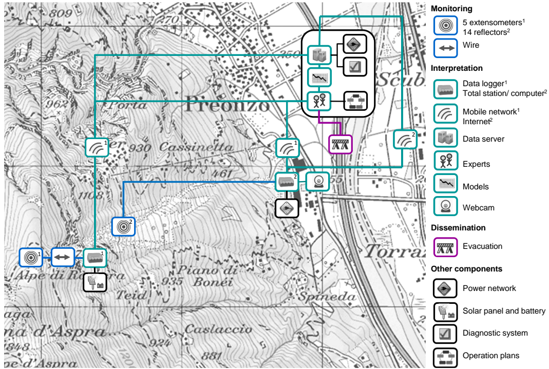
Figure 5. System sketch of the rockslide warning system in Preonzo including partly automated procedures in the monitoring, interpretation, and dissemination unit. (Figure based on pixmaps 2015 swisstopo (5704 000 000).)
