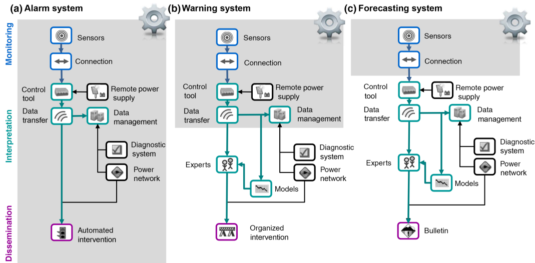
Figure 2. Classification of EWSs: each EWS class includes typical system components facilitating the monitoring and interpretation of data, and the dissemination of warnings. Automated system parts are highlighted in grey.
