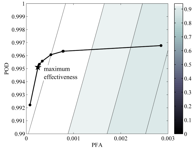
Figure 17. The effectiveness of the Illgraben alarm system could be quantified as a function of POD and PFA; i.e. the reliability (Sättele et al., 2015a).
