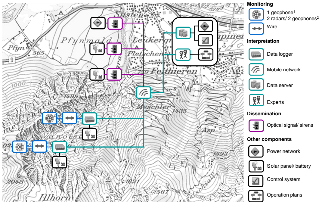
Figure 4. System sketch of the debris flow alarm system in the Illgraben catchment including automated procedures in the monitoring, interpretation, and dissemination unit. (Figure based on pixmaps 2015 swisstopo (5704 000 000).)
