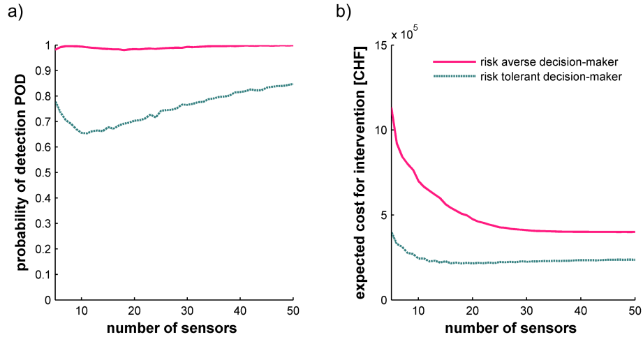
Figure 15. The reliability (POD) and costs for intervention are modelled for two decision-makers and a varying number of initial sensors: (a) the less risk-tolerant decision-maker reaches high values of POD independent of the number of sensors; the risk-tolerant decision-maker only reaches a POD up to 0.85; (b) the more risk-tolerant decision-maker creates lower expected costs, which reach a minimum of CHF 215 000 with around 20 sensors or more; for details see Sättele et al. (2015b).
