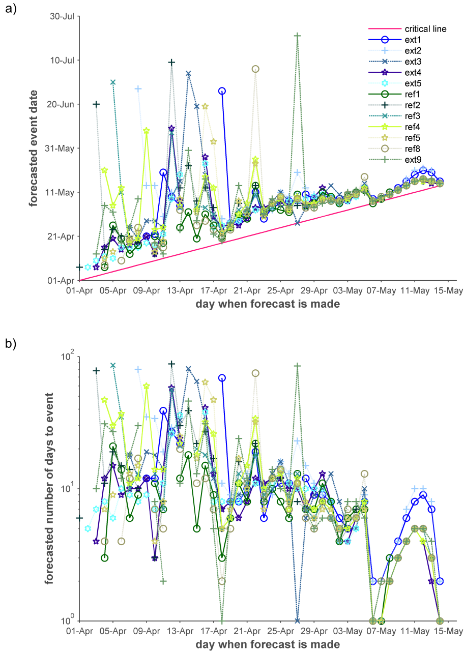
Figure 14. In Preonzo, the model accuracy increases with decreasing lead time. In April, sensor forecasts made with the inverse velocity model vary strongly among different sensors. On May 14, 10 out of 12 sensors predict the event correctly for the next day (Sättele et al., 2015b).
