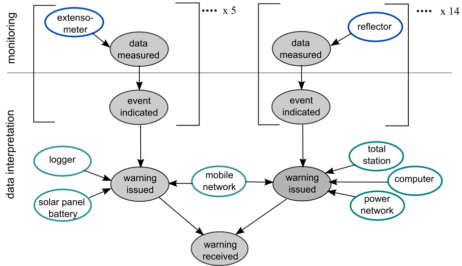
Figure 10. The BN to model the technical reliability achieved in the automated part of the Preonzo warning system is shown. The redundant monitoring unit includes 5 extensometers and 14 reflectors. In the data interpretation unit, warning information is issued automatically to decision-makers. For details, see Sättele et al. (2015b).
