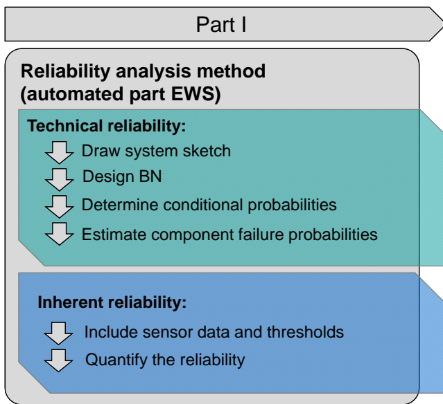
Figure 8. Part I includes six steps to model the technical and inherent reliability of automated EWSs.
