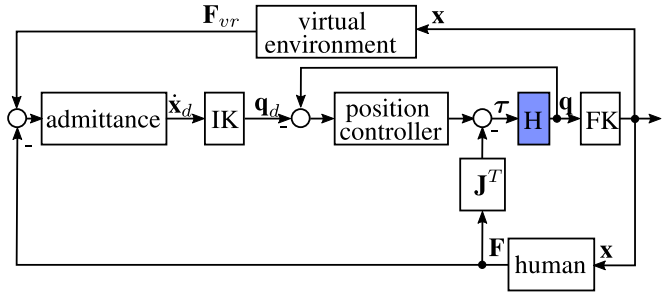
Fig. 4. Admittance control scheme that determines the interaction of the haptic interface (H) with the virtual environment and the human operator. Forward kinematics (FK) and inverse kinematics (IK) transform between Cartesian and joint space. A low-level position controller sets the desired actuator positions.
