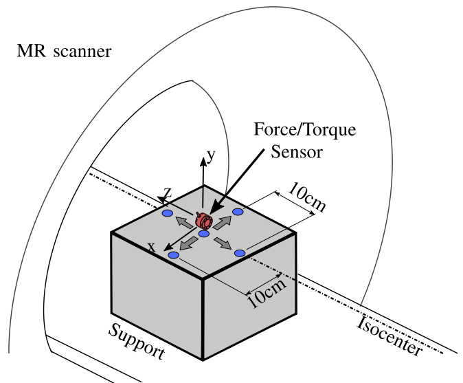
Fig. 12. Setup for force/torque sensor MR-compatibility test.
