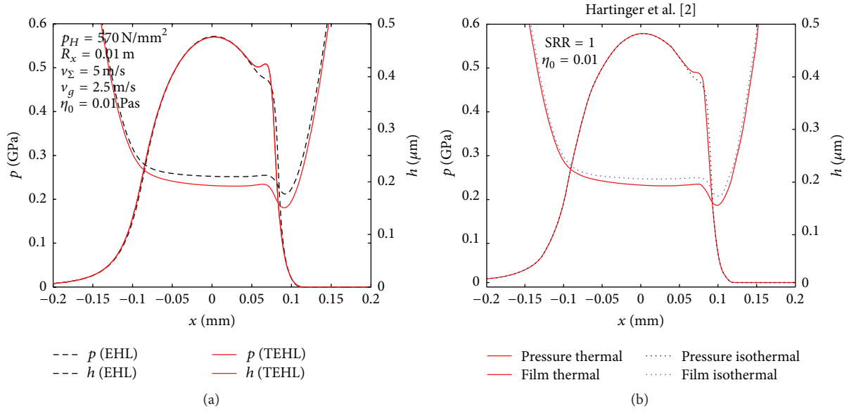
FIGURE 4: Comparison of simulated pressure and film thickness distributions for a thermal (TEHL) and an isothermal (EHL) contact between the TEHL simulation model of this study (a) and the CFD model of Hartinger et al. [2] (b).
