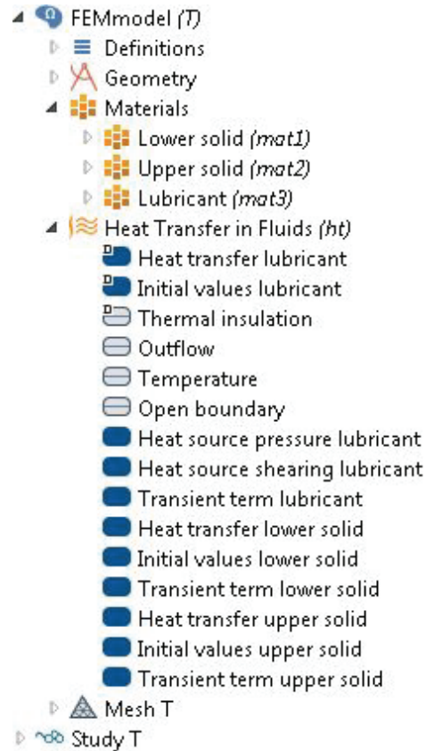
FIGURE 3: FEM-model ( P, H ) for pressure and film thickness calculation with corresponding COMSOL model tree (left) and FEM-model ( T ) for temperature calculation with corresponding COMSOL model tree (right); element numbers are adjusted for presentation purposes.
