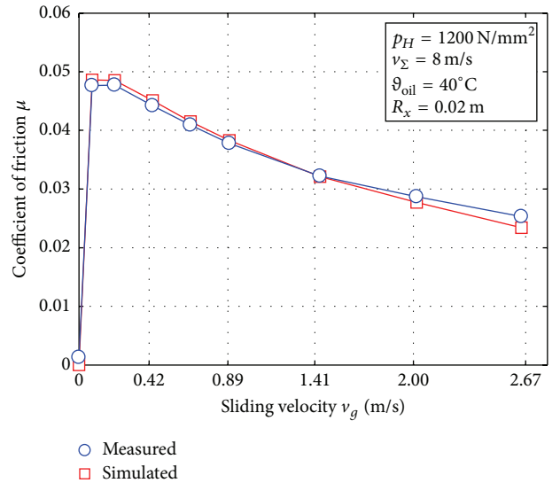
FIGURE 7: Simulated and measured coefficients of friction \mu over the sliding velocity v_g .
