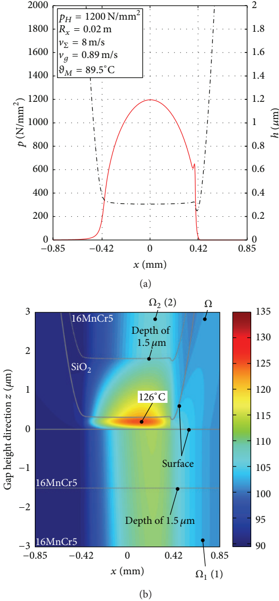
FIGURE 6: Pressure and film thickness (a) and temperature distribution (b) of a TEHL contact with coated ( \text{SiO}_2 ) upper solid acc. to Lohner et al. [27].
