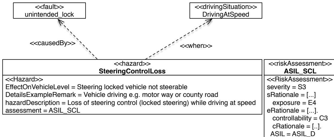
Figure 10. ESCL Hazard Example based on [8]
