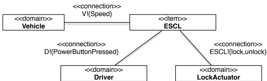
Figure 7. ESCL Context Diagram based on [8]
