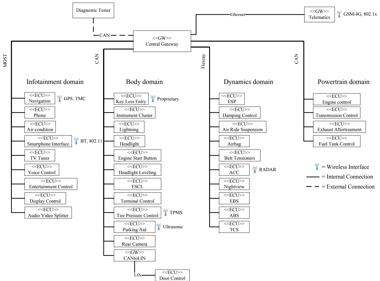
Figure 6. Exemplary Conceptual Automotive Architecture
