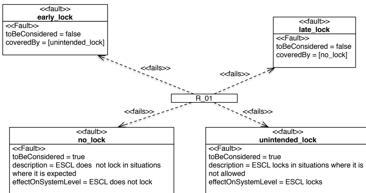
Figure 8. ESCL faults based on [8]
