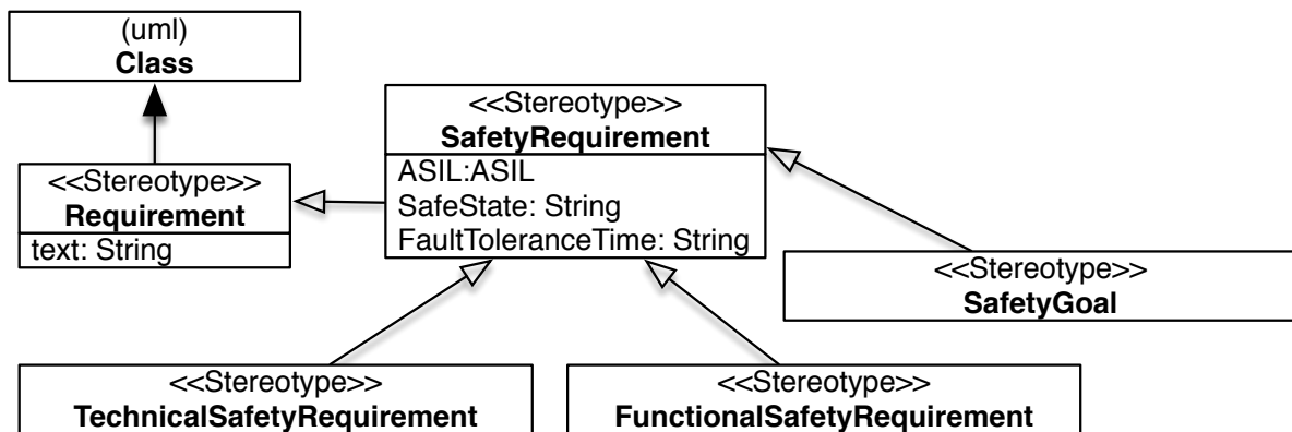
Figure 3. Requirements based on [8]
