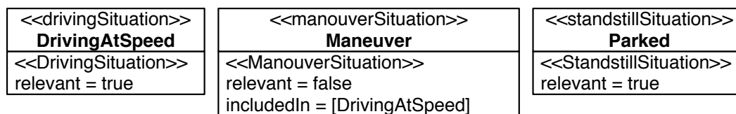
Figure 9. ESCL Situations based on [8]
