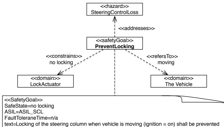
Figure 11. ESCL Safety Goal based on [8]
