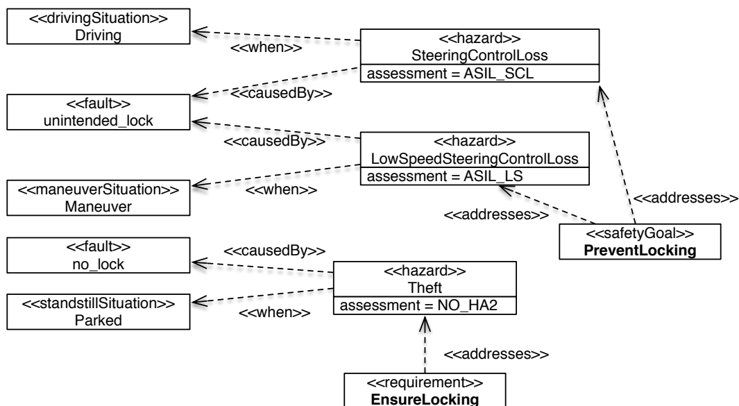
Figure 12. Safety Goal - Hazard - Fault Relations based on [8]
