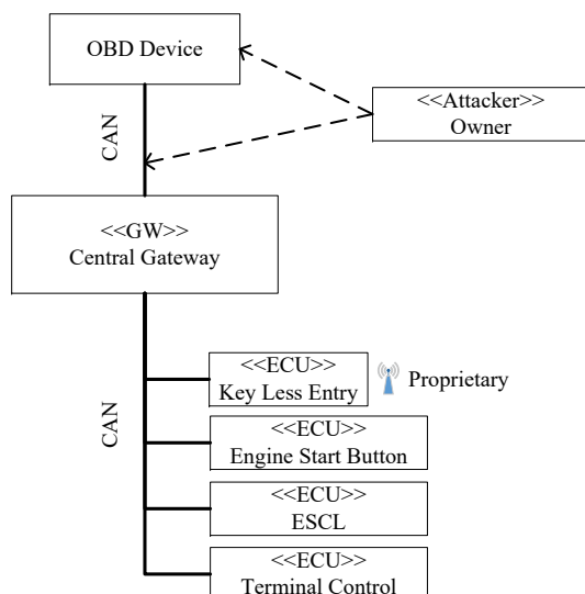
Figure 14. Sub-architecture and attacker type Owner with physical access
