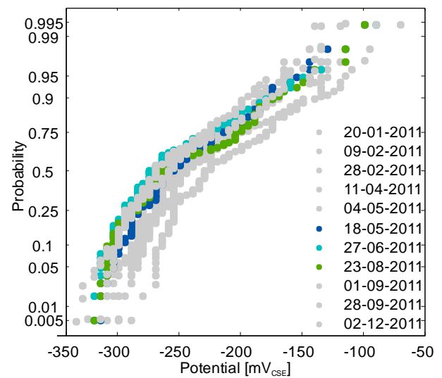
Figure 14. Probability plots of the potential mapping data during rain periods (above) and dry periods (below).
