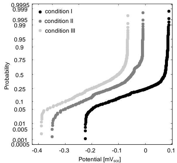
Figure 7. Probability plot of the half-cell potential measurement in the electrolytic pipe under variation of the conductivity.
