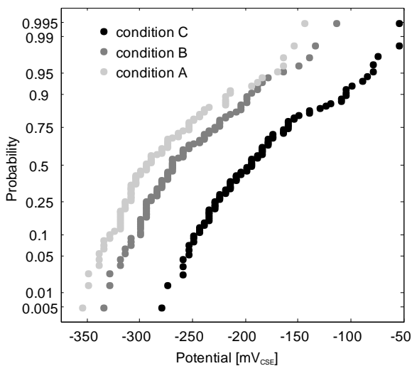
Figure 11. Probability plot under different pre-wetting condition.
