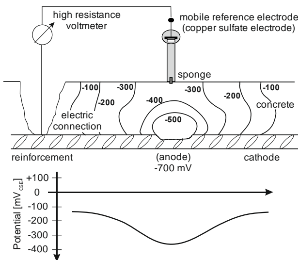
Figure 1. Schema half-cell potential measurement.
