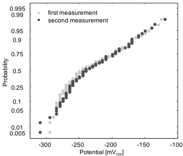
Figure 8. Probability plot of the repeated potential mapping; segments Olympic Stadium.
