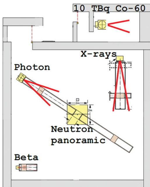
Figure 1. Top view of the calibration hall with the four irradiators and of irradiation room 1 with the photon irradiator.
