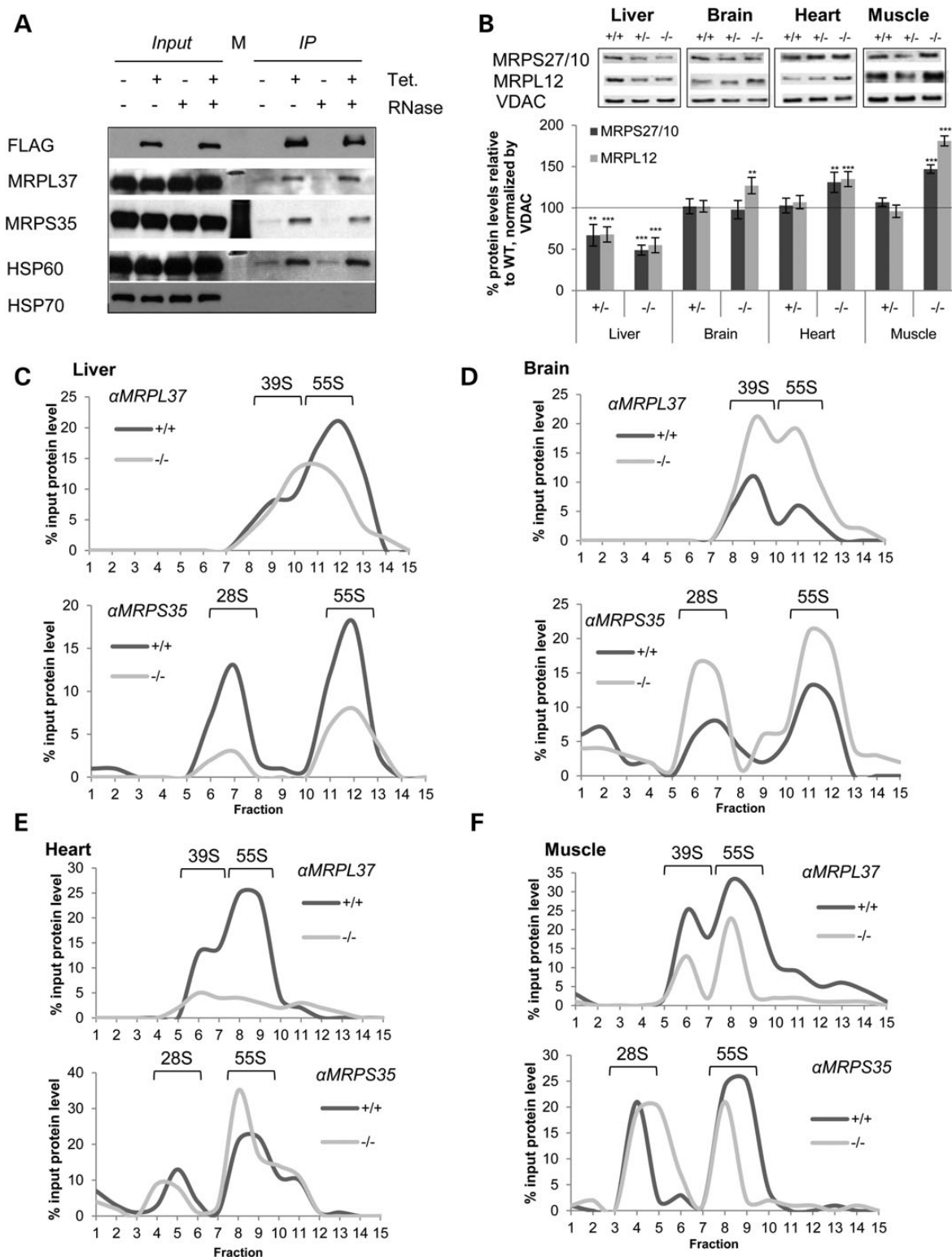
Figure 5. MTO1 interacts with mitoribosomal subunits and affects mitoribosome assembly. (A) Immunoprecipitation of MTO1 from HeLa cells expressing flag-tagged MTO1 from a TET promoter. Immunoprecipitations were performed in the absence and presence of RNase. The eluate was probed by immunoblotting for the presence of the mitoribosomal proteins MRPL37 and MRPS35 as well as for HSP60 and HSP70. (B) Western blot analysis and quantification of mitochondria of WT, heterozygous and homozygous MTO1 mice to assess enzymes connected to the mitochondrial translation. Steady-state levels of mitoribosomal proteins MRPS27/10 and MRPL12 tested. Porin (VDAC) was used as a loading control. Depicted are representative blots. (C-F) Analysis of mitoribosomal assembly by sucrose gradient ultracentrifugation using mitochondrial extracts. Sedimentation of the 28S (small subunit), 39S (large subunit) and 55S (monosome) were determined by western blot analysis. Shown is the quantification of the western blots. The amount relative to the input is depicted. See also Supplementary Material, Figure S4. ** P < 0.01 , *** P < 0.001 .
