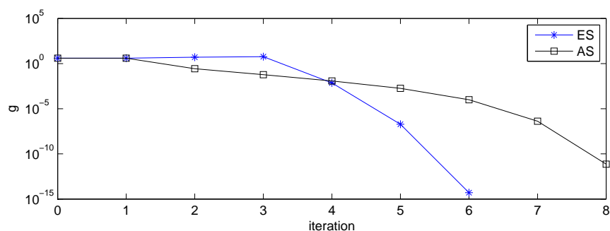
Figure B.4.: Convergence of g for (x_0, y_0) = (-0.5, -1.5)
