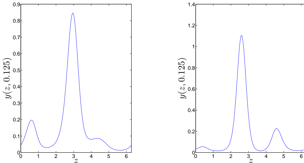
Figure 5.10.: Solutions for node A (left) and B (right) at t = 0.125 .
