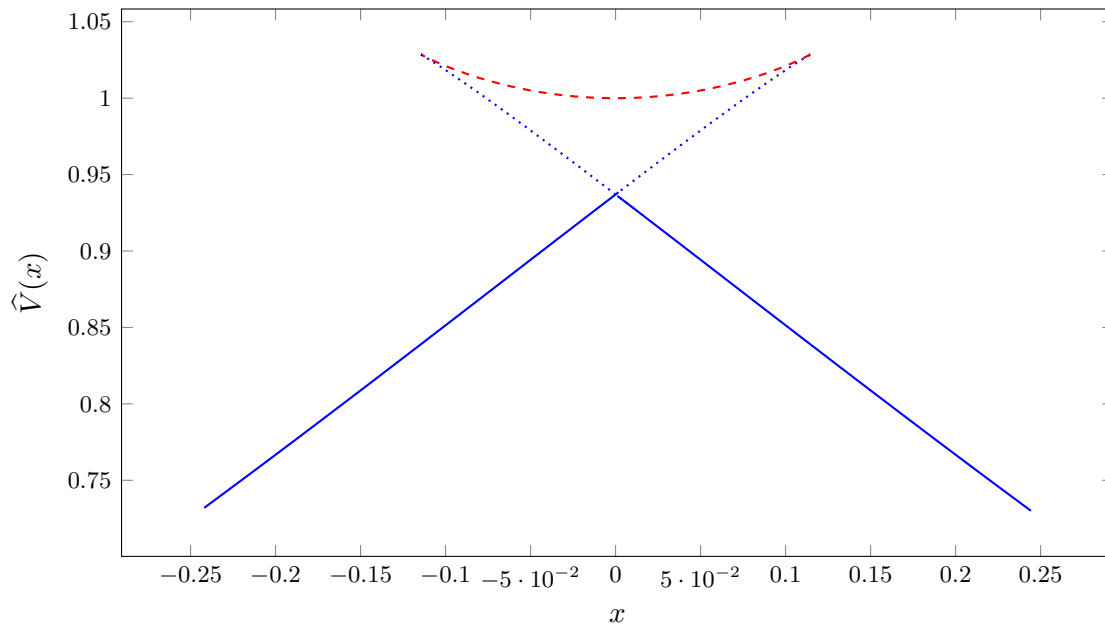
Figure 4.3.: \widehat{V} for T = 1.5 . The actual value function is solid and values of additional, not globally optimal, extrema are dotted for minima and dashed for maxima.
