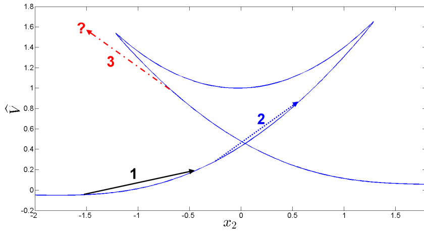
Figure 5.3.: Possible types of homotopy outcomes in Algorithm 5.1, demonstrated on \widehat{V}(0, x_2) from Example 4.10.
