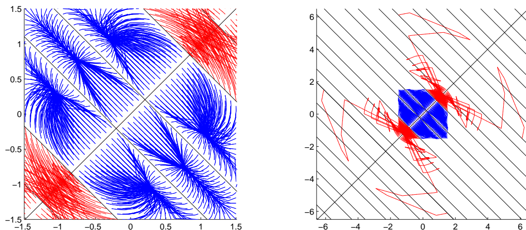
Figure B.3.: Iterates with stepsize control (ES) for several initial values at two zoom levels. Blue paths converge to solutions, red paths converge to singular manifolds, black lines are singular manifolds
