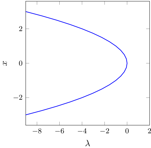
Figure 3.1.: Fold singularity of G(\lambda, x) = \lambda + x^2 .
