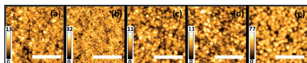
Fig. 3 AFM topography images of the calcined ZnO nanostructured films subjected to THF vapor treatment before the calcination step for (a) 0, (b) 3, (c) 9, (d) 12 and (e) 48 hours. All the images are (2 \times 2) \mu\text{m}^2 and the scale bar for all the images is 1 \mu\text{m} long. The color bar as insets in the images indicates the height of the nanostructures in nm.
