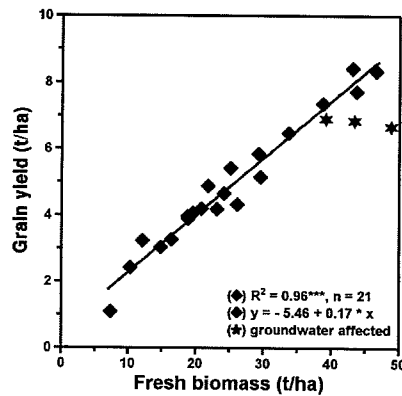
FIGURE 2: Relationship between winter wheat biomass at the development stage of early yellowing and the grain yield
