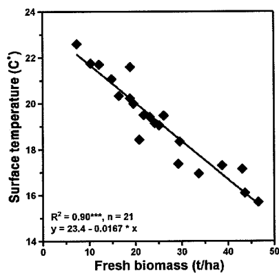
FIGURE 5: Relationship between winter wheat biomass at the development stage of early yellowing and canopy surface temperature
