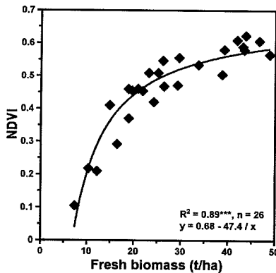
FIGURE 4: Relationship between winter wheat biomass at the development stage of early yellowing and the normalized differential vegetation index (NDVI)
