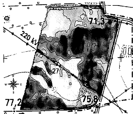
FIGURE 6: Map of plant available water capacity of the root zone as it varies across the reference field 1 (<50 mm = black to >250 mm = white)
