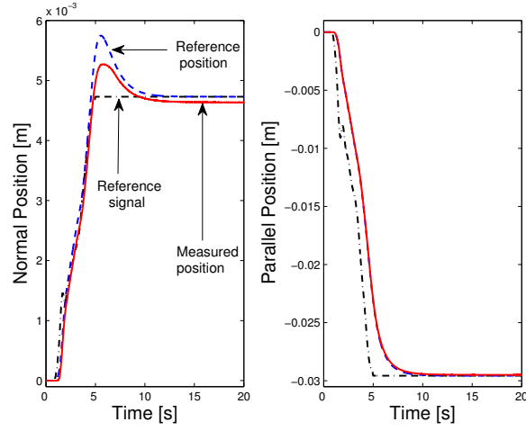
(a) Multiple-Input ESC-MRAC
