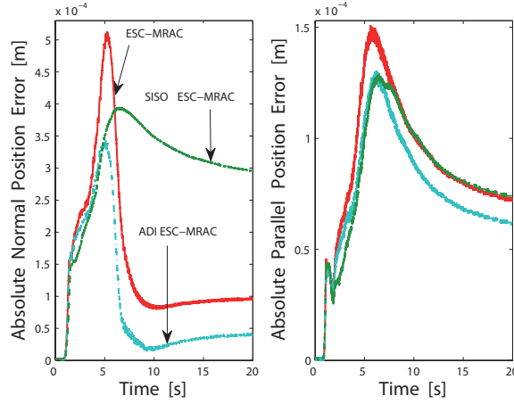
Figure 9: Error between reference and measured position of: (solid red line) Multiple-Input ESC-MRAC, (dashed green line) SISO ESC-MRAC and (dash-dot turquoise line) Multiple-Input ADI ESC-MRAC, in the two directions of movement.
