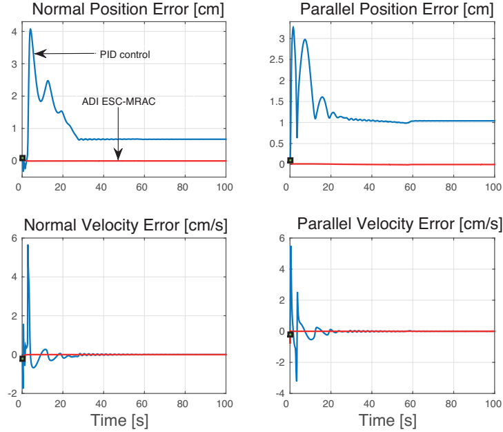
Figure 6: Comparison of Multiple-Input ADI ESC-MRAC with PID control for the test case 1: state tracking error of (red) ADI ESC-MRAC and (blue) PID control. Green markers are used to highlight the initial error value of ADI ESC-MRAC. All signals are expressed with respect to time in sec.
