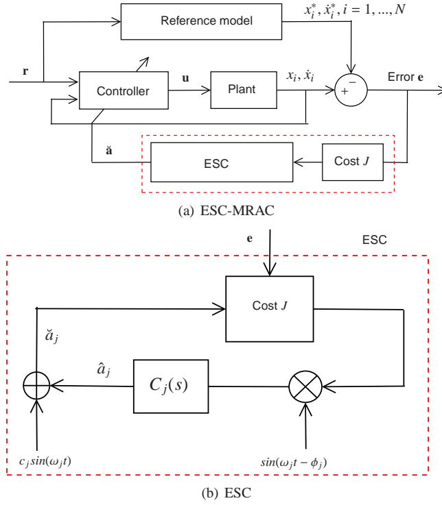
Figure 2: (a) General ESC-MRAC control scheme of a multiple-input system. The plant's state vector [x_1 \ x_2 \ \dots \ x_N \ \dot{x}_1 \ \dot{x}_2 \ \dots \ \dot{x}_N] is ensured to track the reference state vector [x_1^* \ x_2^* \ \dots \ x_N^* \ \dot{x}_1^* \ \dot{x}_2^* \ \dots \ \dot{x}_N^*] through appropriate design of the control law \mathbf{u} . The control parameter vector \check{\mathbf{a}} = \{\check{a}_1, \dots, \check{a}_M\} is adapted based on the minimization of the cost J through PESC. (b) PESC adaptation loop which applies on every single parameter a_j, j = 1, \dots, M where M is the total number of the adaptive parameters.
