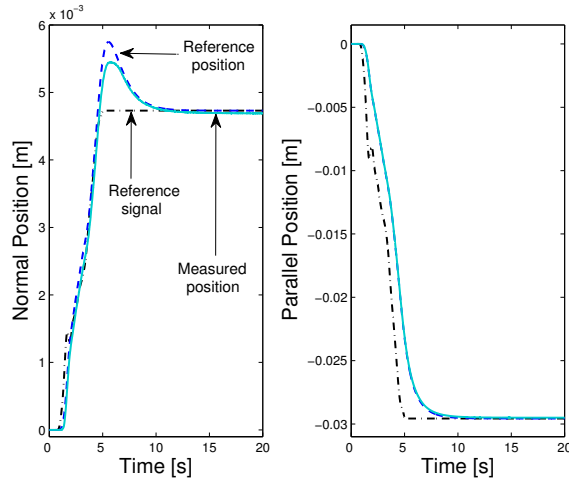
Figure 8: Position tracking by Multiple-Input ADI ESC-MRAC: (dash-dot black line) reference signal, (dashed blue line) reference position, (solid turquoise line) measured position.
