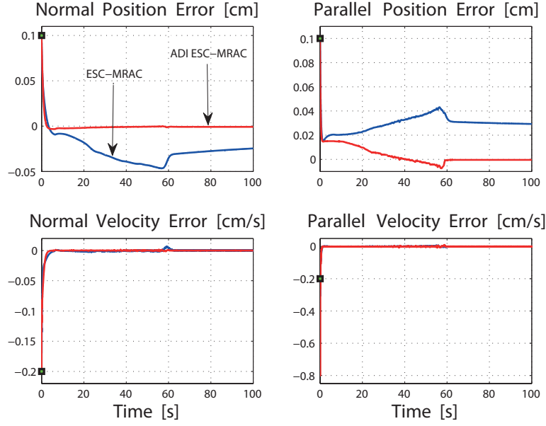
Figure 4: Test case 1: comparison of Multiple-Input ADI ESC-MRAC with Multiple-Input ESC-MRAC. State tracking error of (red) ADI ESC-MRAC and (blue) ESC-MRAC. Green markers are used to highlight the initial error value of ADI ESC-MRAC. All signals are expressed with respect to time in sec.
