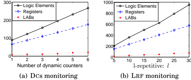
Fig. 13: Results of resource usage after synthesis
