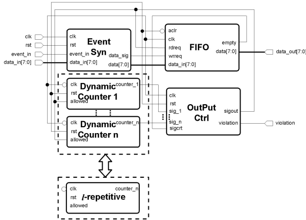
Fig. 12: Block diagram of the FPGA testbed
