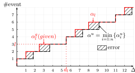
Fig. 7: Arrival curve of periodic burst events (red solid line) that is segmentally repetitive. The black dash line represents a more conservative arrival curve that is the minimum of a set of staircase functions and is used in DCs monitoring.
