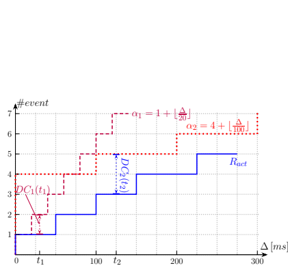
(a) An example for an arrival curve as the combination of staircase functions. The arrival curve is \alpha_{min} = \min(\alpha_1, \alpha_2) . R_{act} is the actual event arrival trace. DC_1(t_1) denotes the potential burst capacity with the constraint of staircase function \alpha_1 at the time t_1 . DC_2(t_2) denotes the potential burst capacity with the constraint of staircase function \alpha_2 at the time t_2 .
