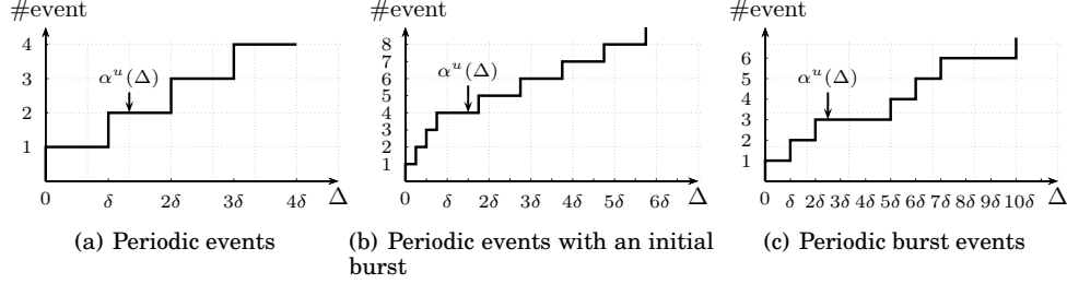
Fig. 3: Arrival curves of three types of event stream.
