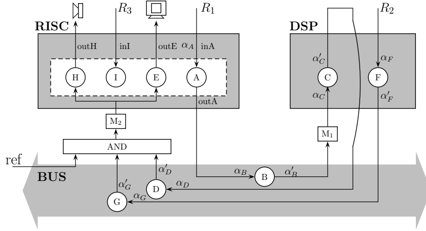
Fig. 8: Analysis model of the MPEG-2 decoder mapped onto an MpSoC platform
