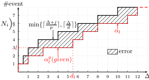
Fig. 4: Arrival curve of periodic events with jitter (black solid line) that is the minimum of two staircase functions. The red dash line represents a more conservative arrival curve that is segmentally repetitive and is used in LRF monitoring. The shadow area shows the error between the arrival curve and the approximated curve.
