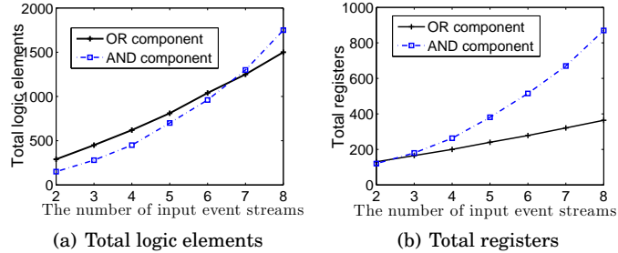
Fig. 14: Resource usage of different monitoring method IPs
