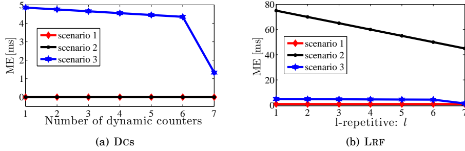
Fig. 10: The monitoring accuracy of DCs and LRF at M_1 w.r.t., the number of counters and the number of events in the repetitive segment, respectively
