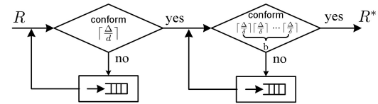
Fig. 6: The flow of monitoring periodic burst arrival events.
