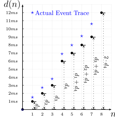
(b) An example of an l -repetitive minimum distance function. The black dot denotes the minimum distance function. The blue star denotes the actual event trace. The interval of successive events should not be smaller than the minimum distance function
