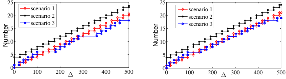
(a) Arrival curve of video frames passing from the BUS to DSP (b) Arrival curve of event stream from the AND component
