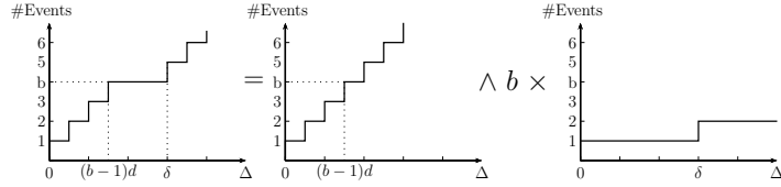
Fig. 5: The diagram of periodic burst pattern equivalence.
