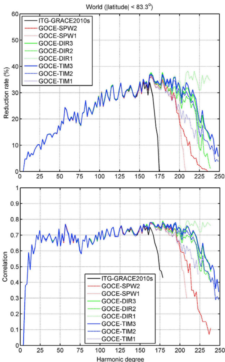
Figure 5. (top) Reduction rates and (bottom) cross-correlation coefficients between RET2011 and GGM gravity as a function of degree n . Evaluation area is -83.3^\circ \leq \delta \leq 83.3^\circ and -180^\circ \leq \lambda \leq 180^\circ .
