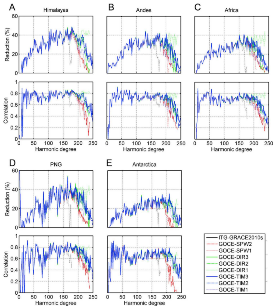
Figure 7. Reduction rates and cross-correlation coefficients between RET2011 and GGM gravity as a function of degree n for five regional study areas: (a) Himalaya ( 20^{\circ} \leq \delta \leq 45^{\circ} and 65^{\circ} \leq \lambda \leq 110^{\circ} ), (b) Andes ( -40^{\circ} \leq \delta \leq 10^{\circ} and -80^{\circ} \leq \lambda \leq -60^{\circ} ), (c) Africa ( -30^{\circ} \leq \delta \leq 30^{\circ} and 10^{\circ} \leq \lambda \leq 40^{\circ} ), (d) Papua New Guinea (PNG) ( -10^{\circ} \leq \delta \leq 0^{\circ} and 130^{\circ} \leq \lambda \leq 150^{\circ} ), (e) Antarctic ( -83.3^{\circ} \leq \delta \leq -70.0^{\circ} and -180^{\circ} \leq \lambda \leq 180^{\circ} ); the legend for all panels is shown in the bottom right.
