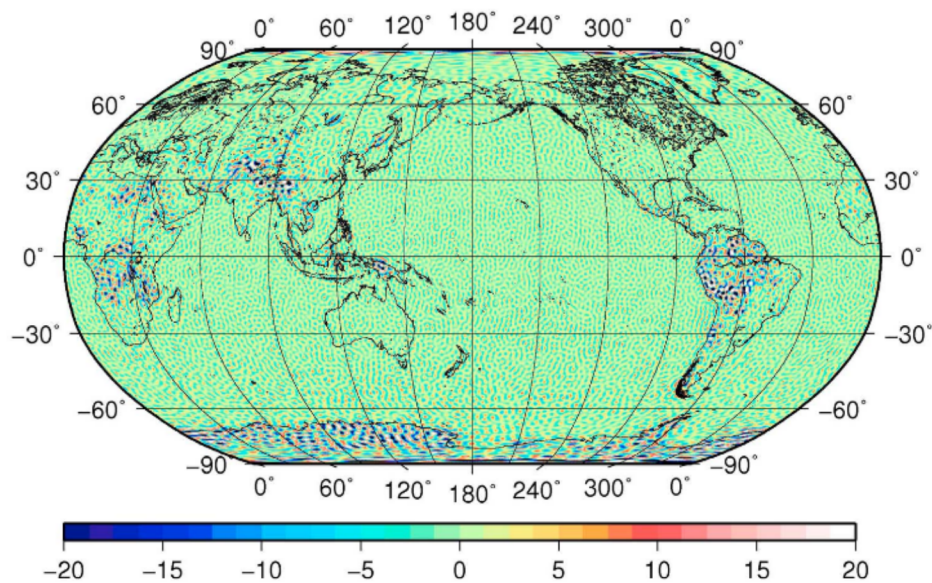
Figure 6. Differences between gravity from EGM2088 and GOCE-TIM2, spectral band 2 to 200, Robinson projection, units in mGal.
