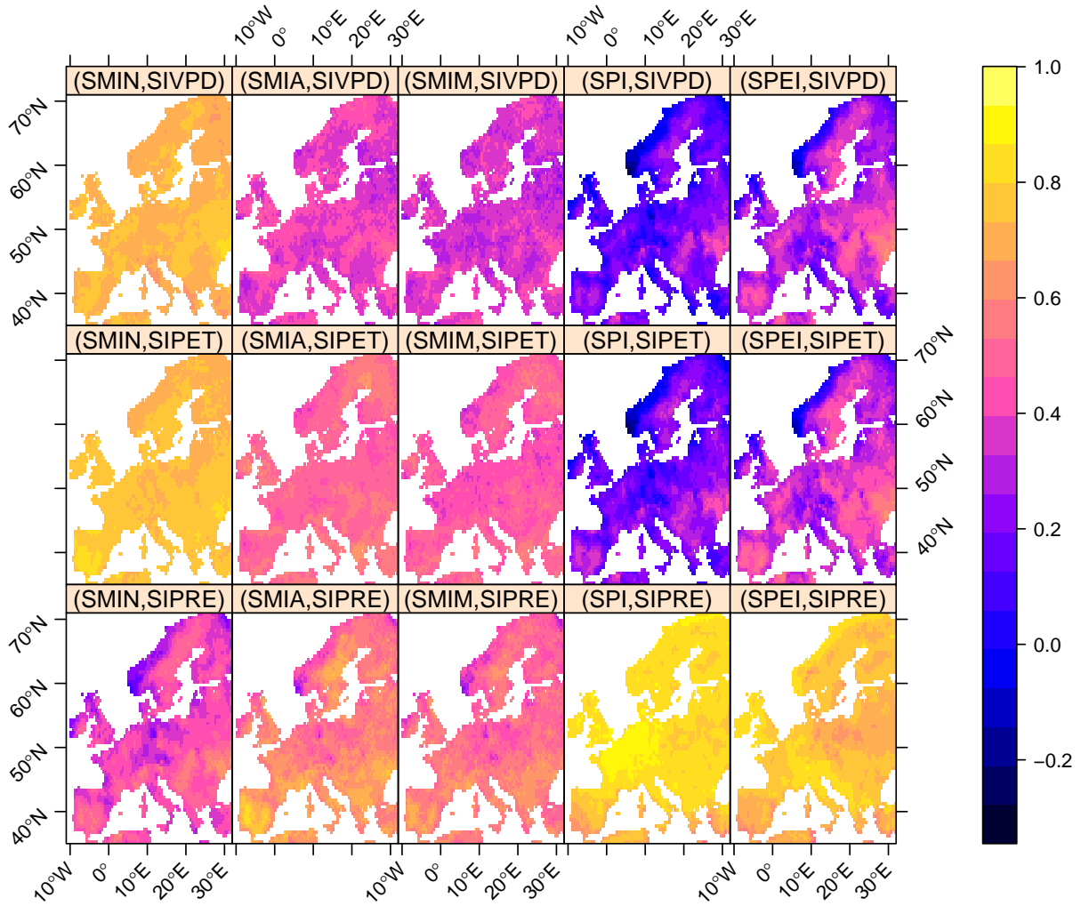
Figure 8: Maps of Kendall's \tau for all combinations of the univariate drought indices SI_6(\text{VPD}) (SIVPD), SI_6(\text{PET}) (SIPET) and SI_6(\text{PRE}) (SIPRE) with the indices SMI_6^N(\mathbf{1}; \text{VPD}, \text{PET}, \text{PRE}) (SMIN), SMI_6^A(\mathbf{1}; \text{VPD}, \text{PET}, \text{PRE}) (SMIA), SMI_6^M(\mathbf{1}; \text{VPD}, \text{PET}, \text{PRE}) (SMIM), SPI_6 (SPI) and SPEI_6 (SPEI).
