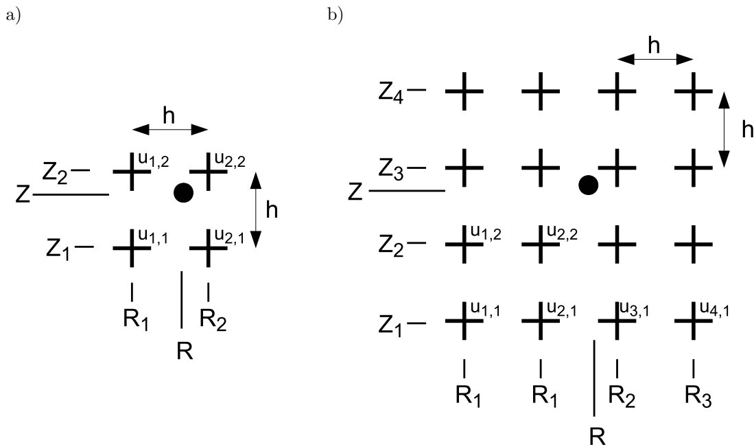
Figure B.1.: a) Interpolation grid for bilinear interpolation, b) for 3rd order bipolynomial interpolation.
