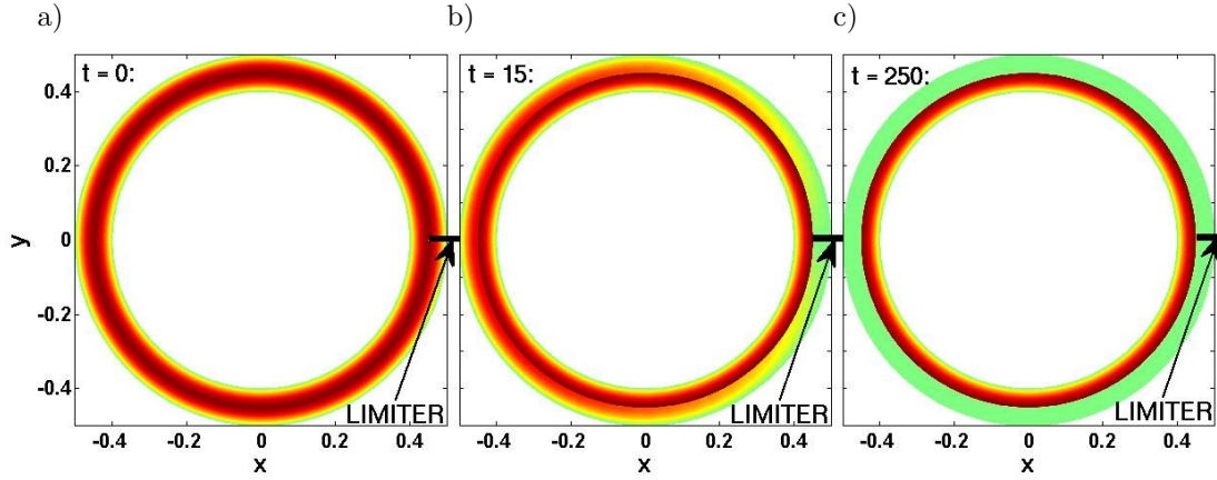
Figure B.8.: Snapshots of a simulation (S-3 scheme performed with N_{pol} = 16 , h = 5 \cdot 10^{-4} , \rho_{min} = 0.4 , \rho_{max} = 0.5 , dt = 1 \cdot 10^{-2} , here shown plane z = 0 ) with an axisymmetric limiter ranging radially half way into the domain. The initial state (a) decays in the open field line region (b). In the final state (c) the mode has decayed completely in the open field line region, whereas it remains stable in the closed field line region leaving a jump in the radial direction.
