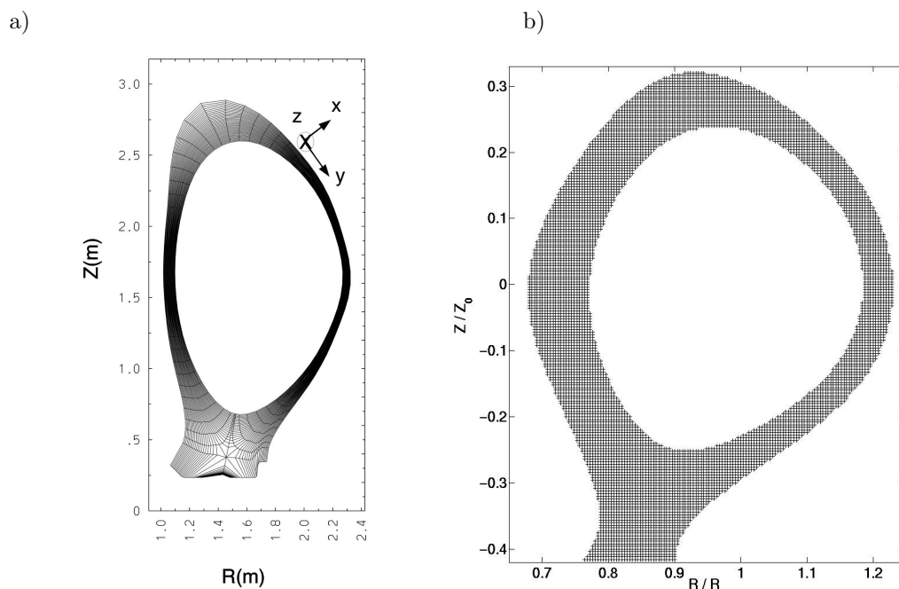
Figure 1.4.: a) Numerical grid as used in the BOUNDary Turbulence code BOUT [37]. Note the special role of the X-point in the grid, which is connected to eight cells, instead as the usual four cells. Moreover there is a huge resolution imbalance between midplane and X-point region. b) Numerical grid as used in the here newly developed code GRILLIX. The X-point is treated as any other grid point and the resolution is homogeneous within poloidal planes.
