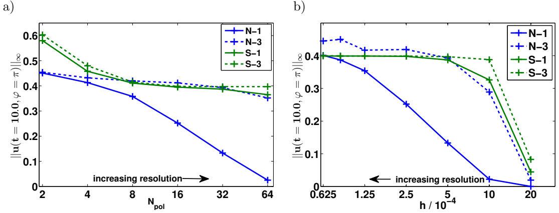
Figure B.3.: Convergence test with blob. The maximum value at the opposed plane \|u(t = 10.0, \varphi = \pi)\| of the initial blob ( R_c = 0.88, Z_c = -0.29, R_w = Z_w = 8 \cdot 10^{-3} ) is plotted against resolution. a) In dependence on toroidal resolution for fixed poloidal resolution of h = 5 \cdot 10^{-4} , b) in dependence on poloidal resolution for fixed toroidal resolution of N_{pol} = 32 . Time step was held constant at \Delta t = 1 \cdot 10^{-2} . For snapshots which illustrate the diffusion of this blob see also figs. 3.13 and 3.15 in section 3.8.
