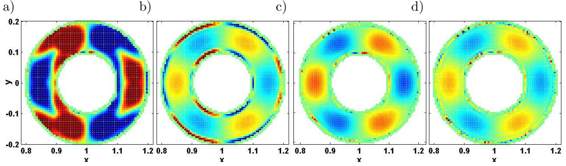
Figure 3.8.: Difference between analytic and numeric solution u^{an}(t_e) - u^{num}(t_e) of a r = 1 , m = 3 , n = 1 mode ( t_e \approx 0.3 ) at z = 0 . a) N-1 , b) N-3 , c) S-1 , d) S-3 . Parameters were q = 3.4 , N_{pol} = 32 , h = 6 \cdot 10^{-3} . Colour code is from -0.01 (dark blue) to +0.01 (dark red).
