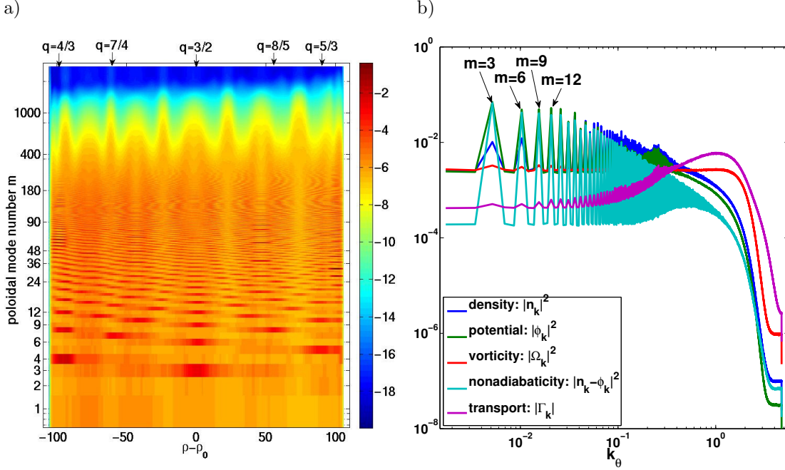
Figure 5.5.: Poloidal amplitude spectra of demonstration simulation averaged between t = 10\,000 - 14\,000 over 801 snapshots. a) Poloidal spectrum of potential, \log |\phi_{k_\theta}|^2 , in dependence on flux surface label. b) Poloidal amplitude spectra at center of flux shell ( \rho = \rho_0 ).
