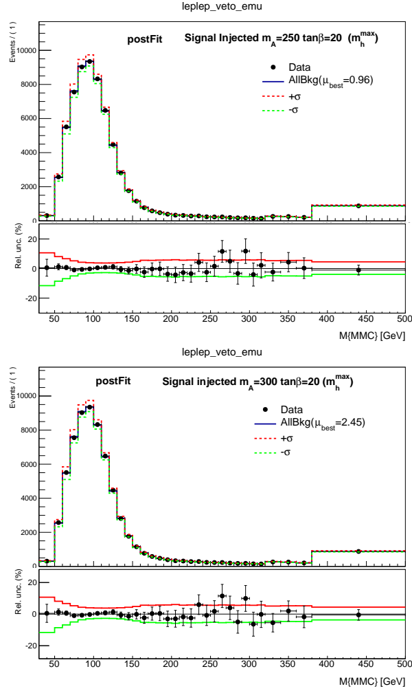
Figure C.8.: Post-fit m_{\tau\tau}^{MMC} mass distribution for the veto category final selections. A signal is injected with m_A = 250 (top) and m_A = 300 (bottom) for \tan\beta = 20 assuming m_h^{max} scenario. The 1\sigma bands represent the statistical and systematic uncertainties.
