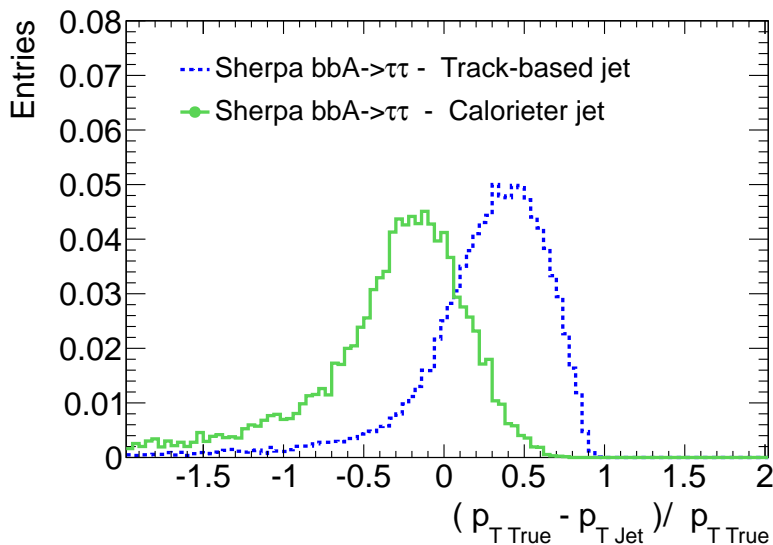
Figure 6.2.: Distribution of transverse momentum residuals relative to the true value P_{T\text{true}} , shown separately for the calorimeter and track-jets.
