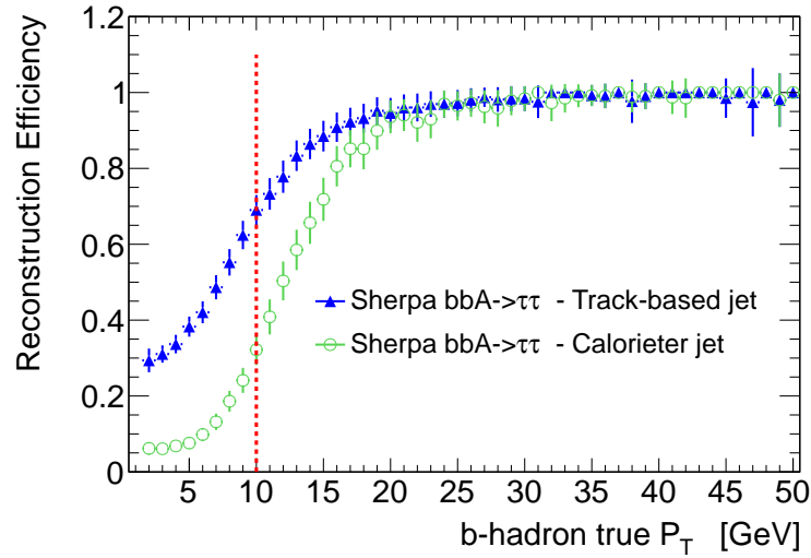
Figure 6.3.: b-hadron reconstruction efficiency for track-jet and calorimeter jets as a function of the true b-hadron p_T . Note that calorimeter and track-based jet are required to have at reconstruction level p_T > 7 and 2 GeV, respectively. A fair comparison in this plot is only possible for p_T > 10 GeV.
