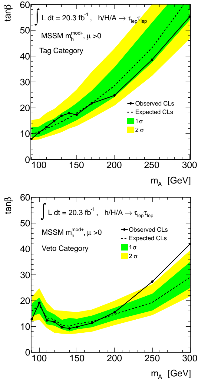
Figure 5.21.: Expected and observed exclusion limits at the 95% CL_s confidence-level for MSSM Higgs bosons production interpreted in the m_A - \tan \beta parameter space of the m_h^{mod} scenario in the b-tagged (top) and b-vetoed (bottom) category.
