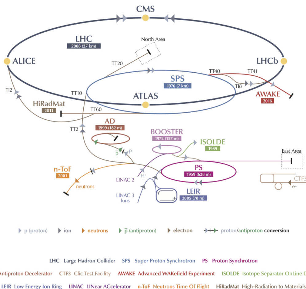
Figure 3.1.: Illustration of the CERN accelerator complex [64]. The acceleration of the protons starts in Linac2 followed by the Booster. The Proton Synchrotron (PS) and the Super Proton Synchrotron (SPS) further accelerate the protons until their final injection into the LHC, where they acquire their final collision energy.
