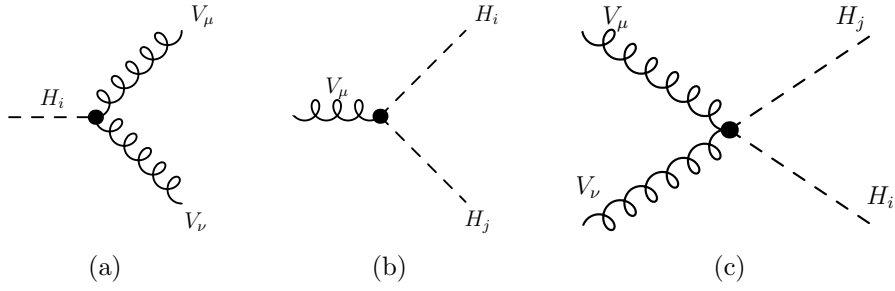
Figure 2.1.: Feynman diagrams for the couplings of (a) one Higgs boson and two gauge boson fields, (b) two Higgs bosons and one gauge boson and (c) two Higgs bosons and two gauge bosons in the MSSM [9].
