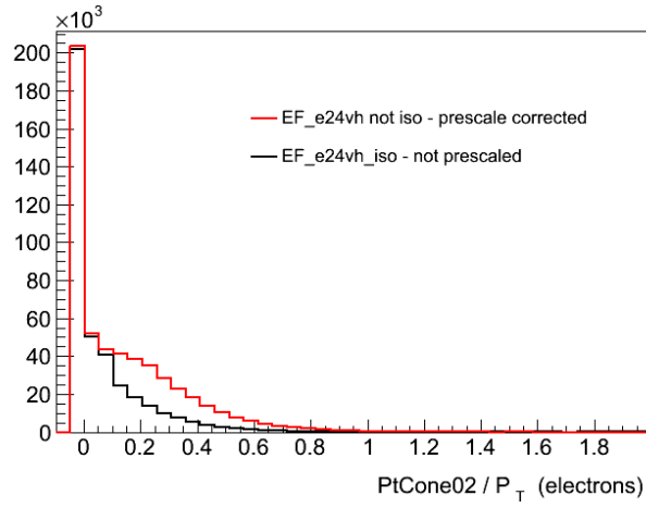
Figure A.1.: p_T(\text{cone}) / p_T distribution for the analysis standard trigger and its cor- rеспective without isolation requirement, this second trigger is rescaled according to prescales information.
