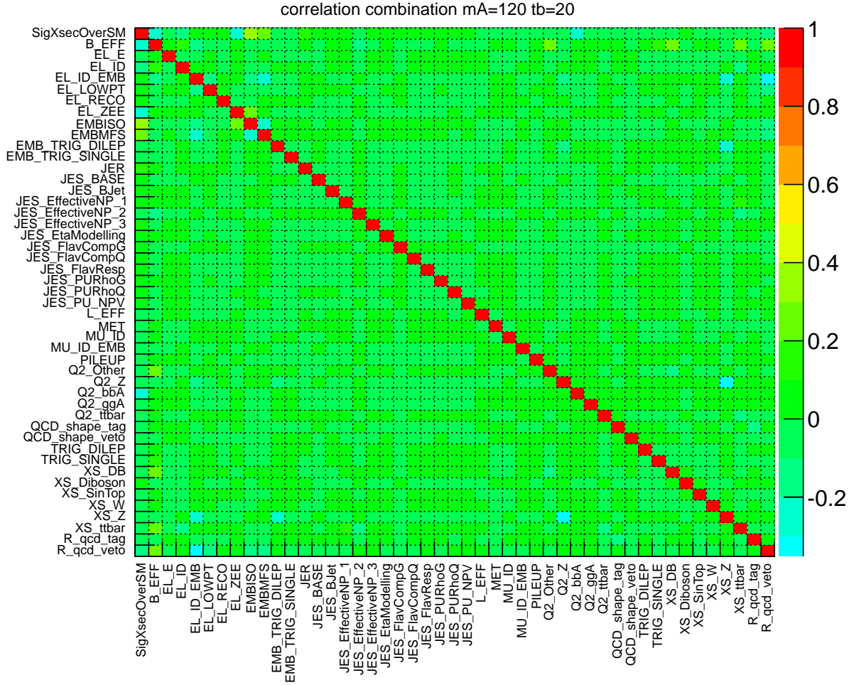
Figure C.3.: Correlation matrix for nuisance parameters considered in the fit. The point m_A = 120 GeV and \tan\beta = 20 is considered for the combination of the b-tag and b-veto channels. This correlation matrix is obtained with NuisanceCheck package, using asymptotic approximation.
