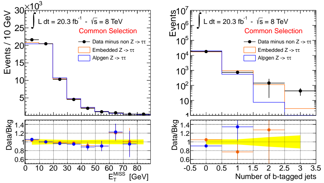
Figure 5.12.: Comparison of the E_T^{miss} (left) and b-tagged jet multiplicity (right) distributions in embedded and in ALPGEN Z/\gamma^* \rightarrow \tau\tau events after the common selection. Data are superimposed after subtracting the contributions of non- Z/\gamma^* \rightarrow \tau\tau processes. The yellow band indicates the total systematic uncertainty of the ALPGEN simulation.
