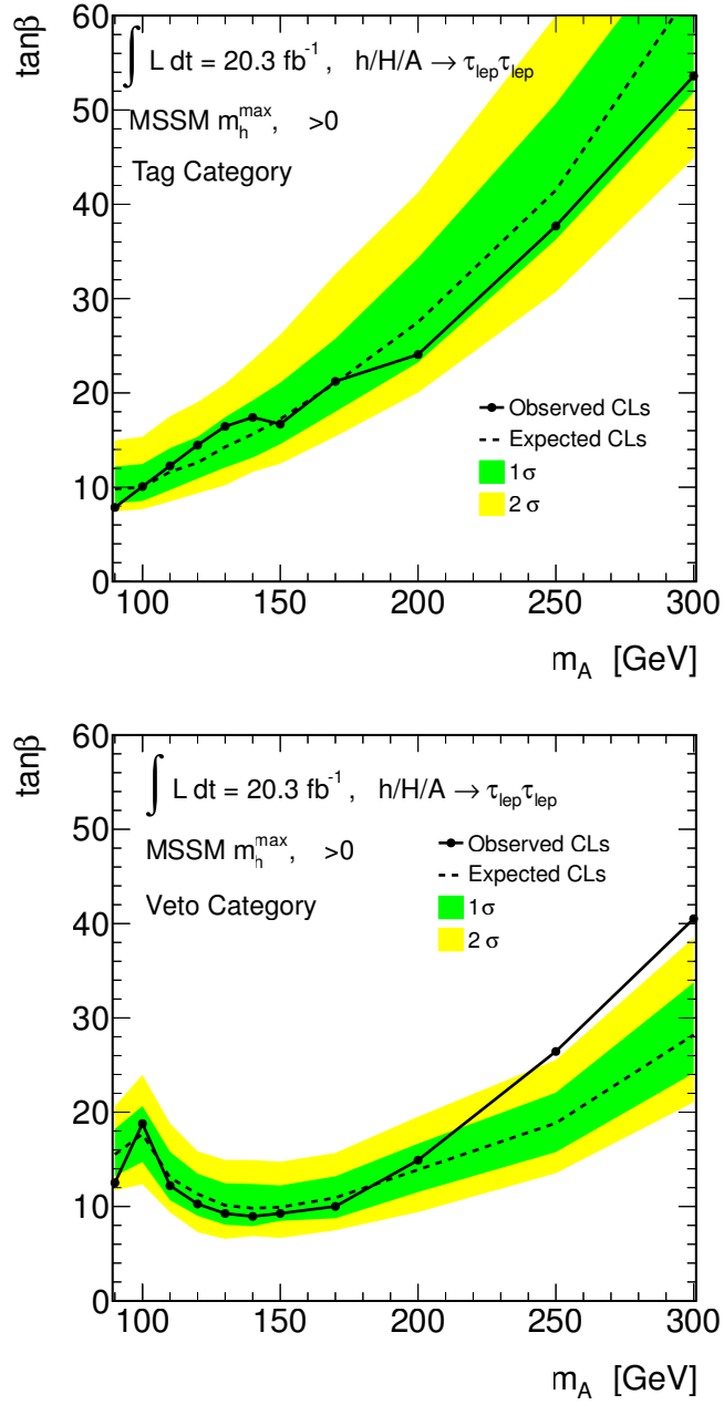
Figure B.2.: Expected and observed exclusion limits at the 95% CL_s confidence-level for MSSM Higgs bosons production interpreted in the m_A - \tan\beta parameter space of the m_h^{\text{max}} scenario in the b-tagged (top) and b-vetoed (bottom) category.
