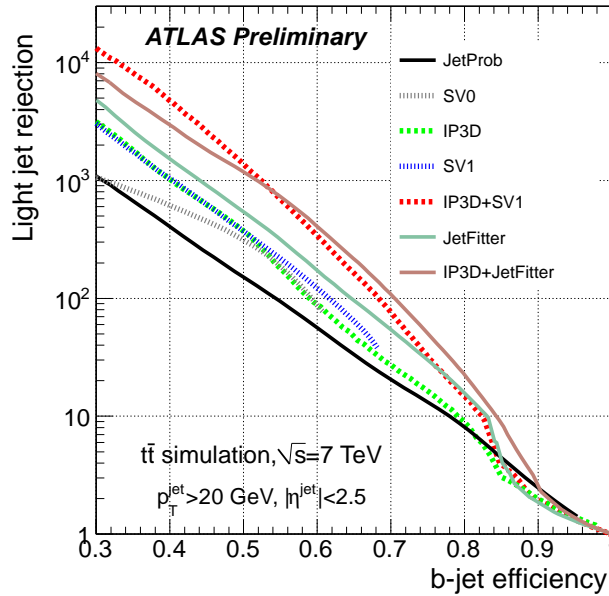
Figure 4.1.: Light-jet rejection as a function of the b-jet tagging efficiency for several different tagging algorithms [121], obtained with simulated t\bar{t} events. The rejection is defined as the inverse of mistagging rate of light jets.
