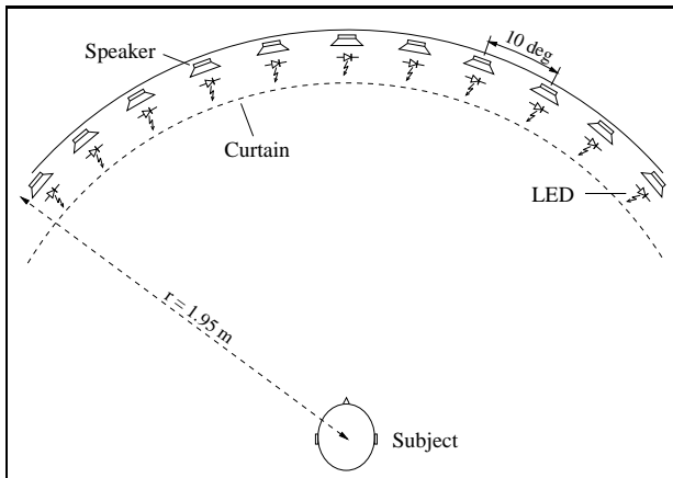
Figure 1. Apparatus.
