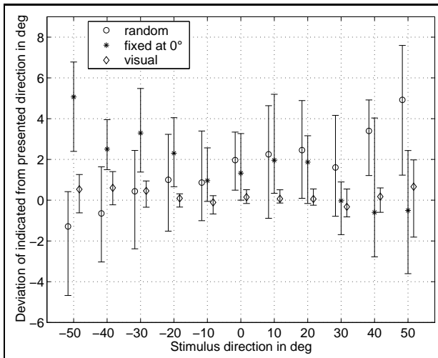
Figure 3. Medians and quartiles of results of localization experiments with wide-band noise pulses and visual stimuli given relative to stimulus position. Exp. 1 (○) : Random initial angle of laser pointer position within \pm 20 deg, Exp. 2 (*) : Fixed initial laser position of \pm 0 deg in front of the subjects, Exp. 3 (◇) : Pointing to remembered visual targets; random initial laser spot position. Angles 50 deg left to 50 deg right were tested in 10 deg increments. The data of Exp. 1 and 3 are shifted horizontally for better distinction.
