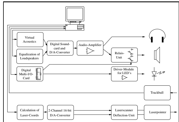
Figure 2. Block diagram of the experimental setup.
