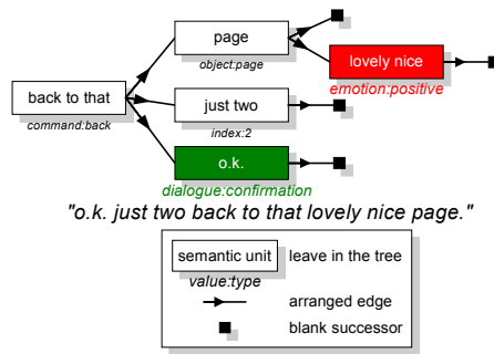
Figure 1: Example of a semantic tree
