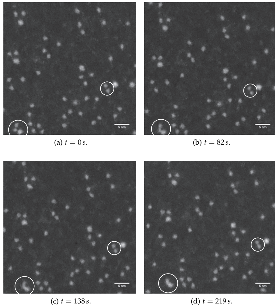
Figure 5.1.6: Series of four subsequent STEM micrographs of 0.03 e/nm^2 Pt_{68} . The images are recorded with an electron beam of 300 kV; two cluster pairs that coalesce as a result of the high beam intensity are marked with circles.
