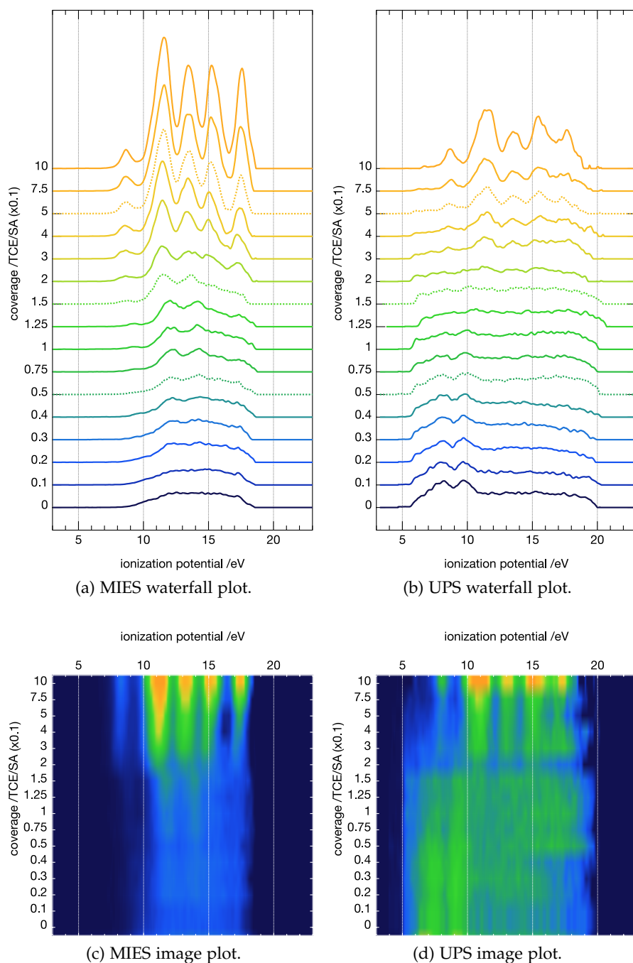
Figure 4.4.7: EE spectra of adsorbed TCE on Pt(111), referenced with respect to the vacuum level of the clean substrate and background corrected. Increasing dosage of TCE from bottom to top; MIES (a) and UPS (b). The bottom spectra show the clean Pt(111) surface. The dashed lines indicate the coverages (0.05, 0.15 and 0.5 TCE/SA) for which the IP energy shift is shown in fig. 4.4.10. Subfigures (c) and (d), show the corresponding image plots for better visibility of the appearance of the TCE peak features for MIES and UPS, respectively. Reprinted (adapted) with permission from [172] - Copyright (2012) Elsevier.
