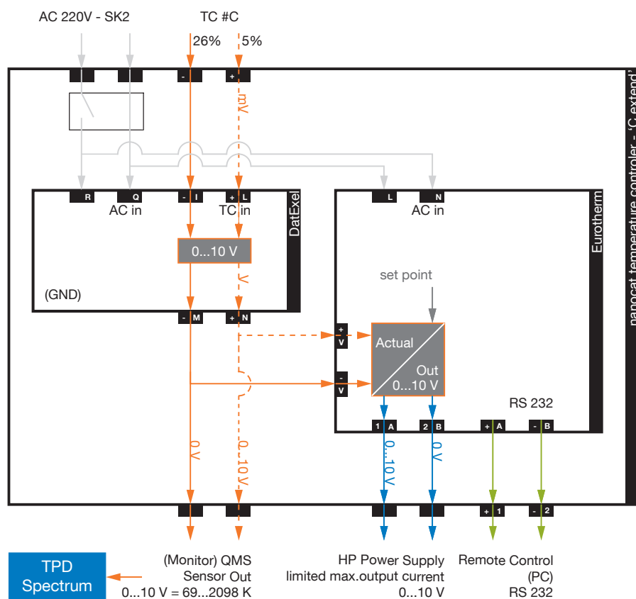
Figure A.1.1: Temperature measurement and control.
