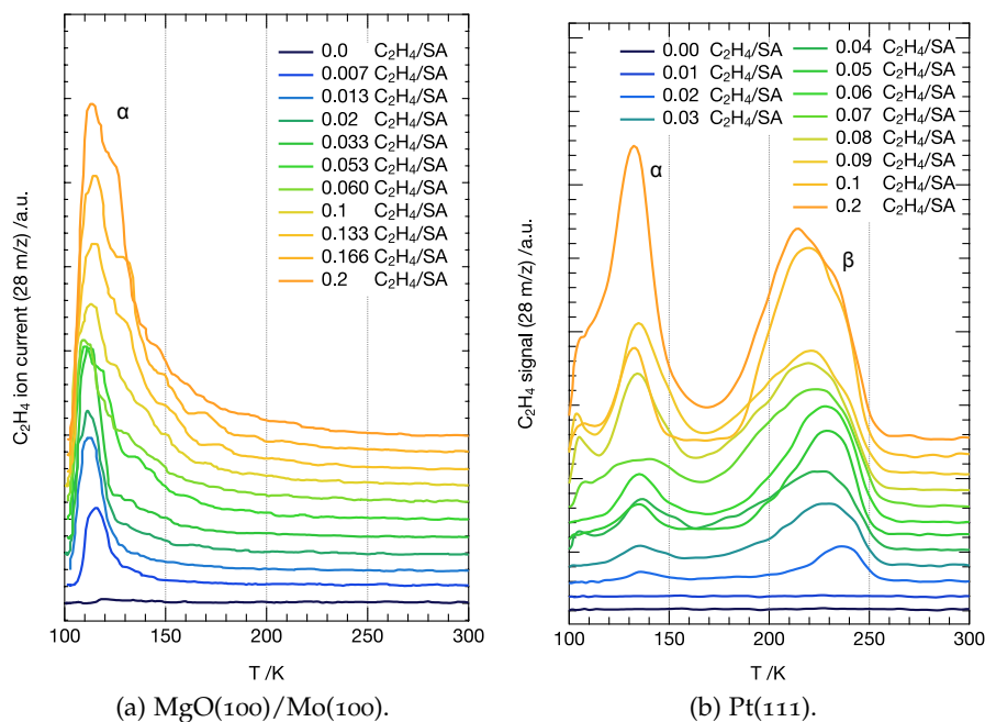
Figure 4.4.16: TPD spectra ( \beta = 2K/s ) of ethene desorption on MgO(100)/Mo(100) (a) and Pt(111) (b). For MgO peak \alpha is assigned to desorption of condensed and physisorbed ethene. In the case of Pt(111) peak \alpha is physisorbed ethene only, while peak \beta is attributed to chemisorbed ethene . Note, that the spectra for Pt(111) were recorded in random order and without cleaning in between dosage and thus do not reflect for each coverage the behaviour on clean Pt(111) .
