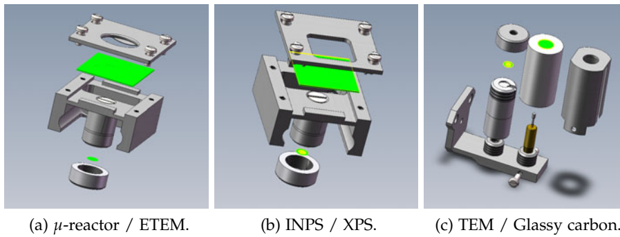
Figure 3.3.2: Holders for sample preparation for ambient experiments, one holder at a time is attached to the manipulator arm by means of two screws. Holders (a) and (b) can accommodate one sample (green) of the indicated type and additionally a TEM sample at a centro-symmetric position; on holder (c) also two TEM samples can be fixed.
