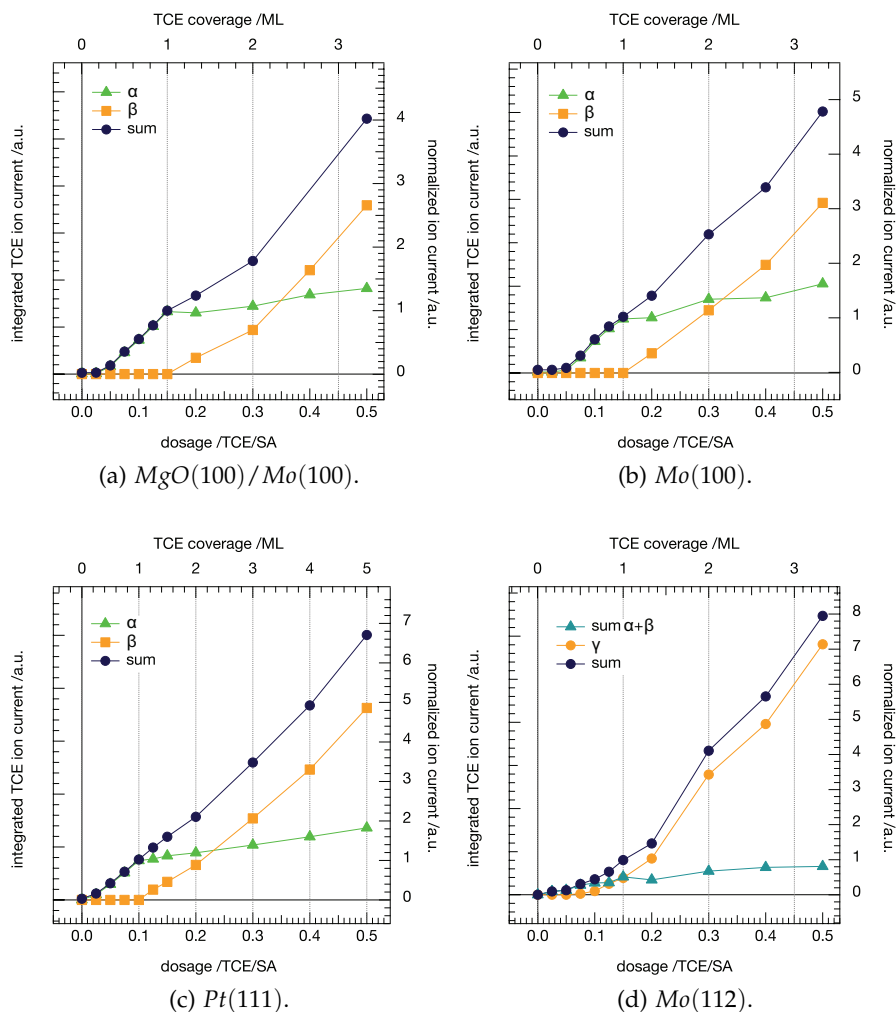
Figure 4.4.2: Integrated areas of the individual peaks and total area for the measured TPD series of TCE on MgO(100) (a), Mo(100) (b), Pt(111) (c) and Mo(112) (d); the scales on the right and on top normalize the determined integrals for comparability of the different surfaces; the dashed lines mark the transition from physisorption to condensation. Reprinted (adapted) with permission from [172] - Copyright (2012) Elsevier.
