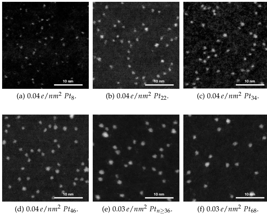
Figure 5.1.1: STEM micrographs ( 30 \times 30 nm^2 ) for Pt_{n,x} ( n > 36 ; x = 8, 22, 34, 46, 68 ) clusters supported on 2 nm carbon. The corresponding coverages are shown in fig. 5.1.2.
