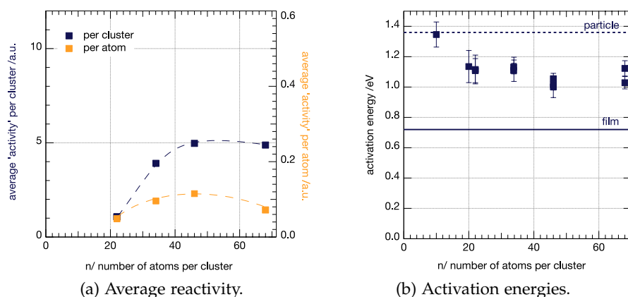
Figure 5.3.6: Average reactivity at full conversion (a) and activation energies (b) for Pt_x as a function of cluster size, for comparison the results of the larger particles (dashed lines) and the thin film (drawn trough lines) are also shown. An indicated error for the activation energies (b) is based on the standard deviation of multiple measurements at the same cluster size; for larger particles and the thin film a similar error holds, is however not explicitly shown. The average reactivity is displayed per cluster (blue) and per cluster atom (orange); the dashed lines serve as a guide to the eye.
