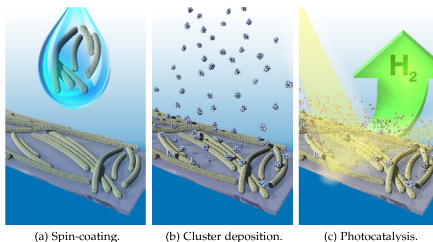
Figure 3.3.6: Schematic representation of the experimental platform for atomic scale insight into photocatalytic nanosystems. Colloidal semiconductor nano crystals ( CdS nanorods) are spin-coated onto ITO substrates (a) followed by deposition of cluster under UHV conditions (b). The resulting samples are investigated for their photocatalytic activity in terms of hydrogen generation efficiency in aqueous solution (c). Reprinted (adapted) with permission from [220] - Copyright (2012) American Chemical Society.
