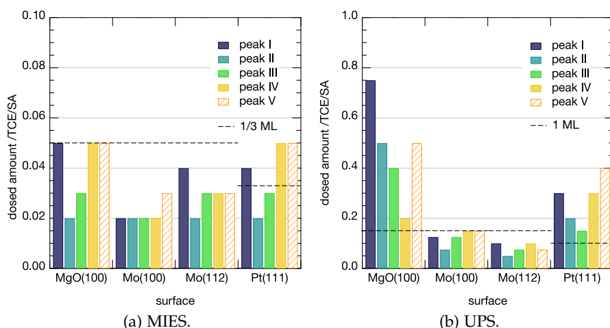
Figure 4.1.2: Minimum amount of TCE necessary to detect the different MOs of the molecule by means of MIES (left) and UPS (right) on the surfaces MgO(100) , Mo(100) , Mo(112) and Pt(111) . The bar graphs are based on the evaluation of the corresponding MIES/UPS spectra recorded as a function of coverage (see sec. 4.4.1) and are based on tab. 4.4.1. The left scale for MIES is increased by a factor of 10 compared to UPS for better visibility, the dashed lines indicate the coverage determined from TPD.
