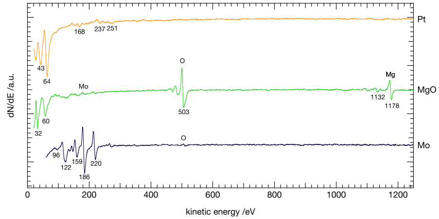
Figure A.1.6: AES spectra of Mo(100), MgO(100)/Mo(100) and Pt(111), modified after [316].
