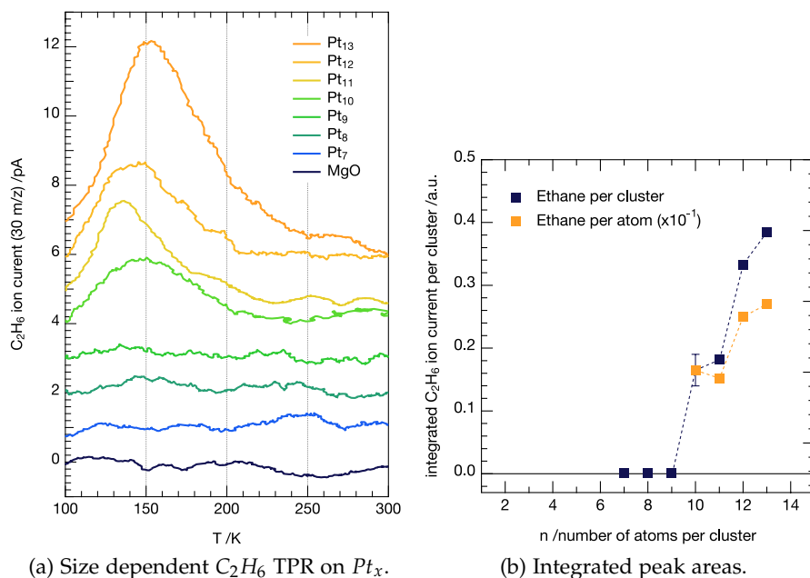
Figure 4.4.27: TPR spectra ( \beta = 2K/s ) of hydrogenation on 0.116 e/nm^2 selected Pt_x ( 7 \leq x \leq 13 ) clusters on MgO(100) . The recorded ion signals ( 30 m/z ) for the pristine support MgO and the different sizes are shown in (a). The corresponding integrated peak area (averaged in case of Pt_{10} and Pt_{11} , because of multiple experiments) are plotted as a function of size (b). The indicated error for Pt_{10} is based on the standard deviation of five TPR measurements; the dashed lines serve as a guide to the eye.
