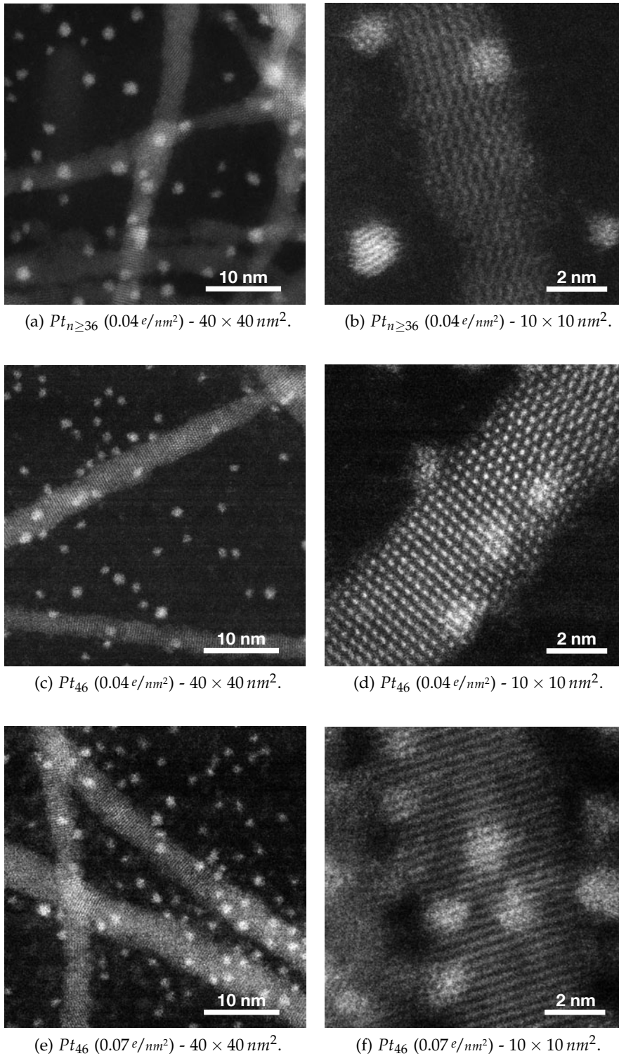
Figure 5.4.2: HAADF-STEM micrographs ( 40 \times 40 nm^2 and 10 \times 10 nm^2 ) of unselected Pt_{n \geq 36} ( 0.04 e/nm^2 ) and two different coverages ( 0.04 e/nm^2 , 0.07 e/nm^2 ) of size-selected Pt_{46} clusters deposited onto CdS NR thin films. For Pt_{n \geq 36} different sizes can be observed, whereas for Pt_{46} the size of the clusters is the same. The amount of clusters fit the expected values. Images at high magnification even allow for resolving atomic structure of rod and Pt clusters. Reprinted with permission from [220] - Copyright (2012) American Chemical Society.
