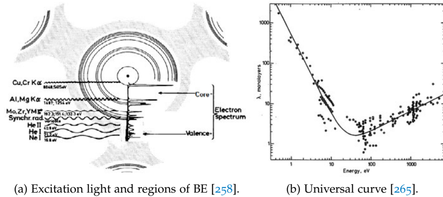
Figure 3.2.2: Regions of BE accessible with different photon sources (a). Solid circles: localized, atom-like orbitals (core electrons). Shaded area: delocalized, molecular orbitals (valence electrons) [258]. Mean free path of electrons in metallic solids as a function of their energy (universal curve) [8, 265, 41] (b).
