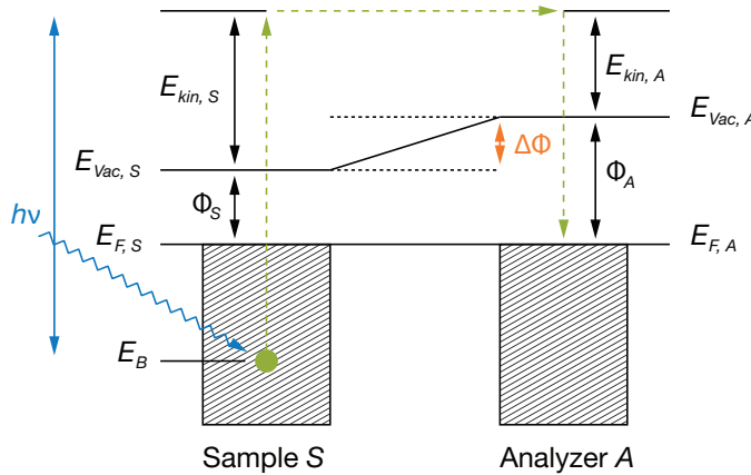
Figure 3.2.4: Energy diagram of the PES process, sample (left) and analyzer (right) are in electrical contact [213].
