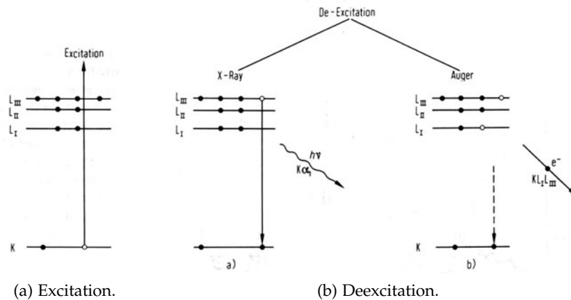
Figure 3.2.3: Deexcitation processes for atomic core holes. a) emission of X-ray radiation, b) emission of an Auger electron [136].
