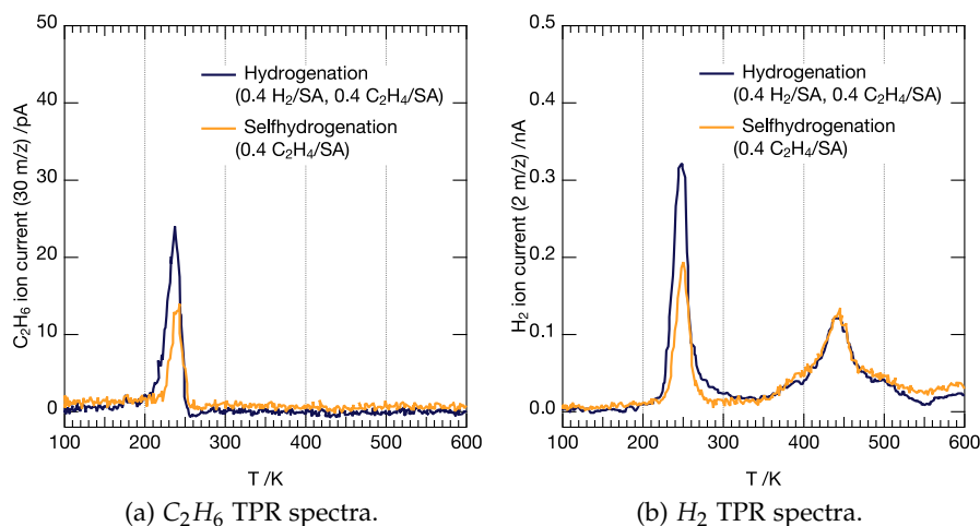
Figure 4.4.25: TPR of C_2H_6 and H_2 desorption on Pt(111) for hydrogenation (blue spectra) and self-hydrogenation (orange spectra). For self-hydrogenation 0.4 C_2H_4/SA of ethene was dosed prior to the TPR, for hydrogenation additionally 0.4 H_2/SA of hydrogen were dosed.
