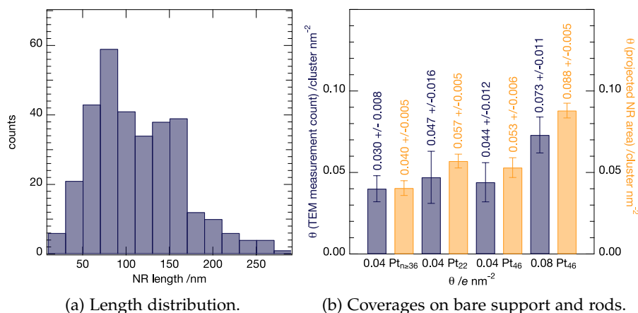
Figure 5.4.4: Length (a) and coverage (b) distribution of the prepared hybrid catalysts. Length distribution of synthesized CdS NRs (a). Rod lengths are measured from a series of TEM images with low magnification (similar to fig. 5.4.1a). Comparison of cluster coverages on graphite support and on CdS NRs (b). For four different samples ( \text{Pt}_{\geq 36} , \text{Pt}_{22} , \text{Pt}_{46} and \text{Pt}_{46} ) the number of clusters found on the bare graphite support (left axis, blue bars) and their number on the projected NR area (right axis, yellow bars) are plotted versus the bottom axis showing the amount obtained by integrating cluster current during deposition. The errors result from variation of the counted numbers within the different STEM micrographs used.
