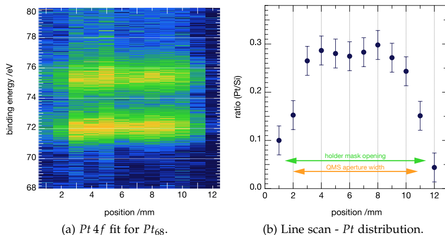
Figure 5.1.10: Image plot of Pt\ 4f signals of 0.029\ e/nm^2\ Pt_{68} (corrected by the Pt to Si ratio) as a function of different spatial positions (a) and spatial distribution of clusters on the support, shown as ratio of the obtained areas from the fitted Si\ 2p and Pt\ 4f signals (b) for each measured position from fig. 5.1.9.
