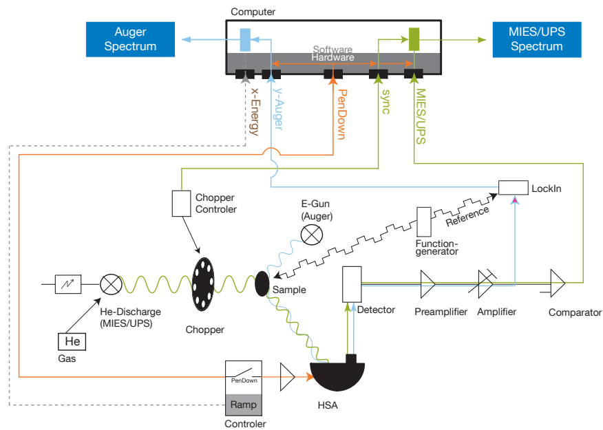
Figure A.1.3: Schematic sketch of the utilized electronic setup for the EES (MIES, UPS and AES) data detection .
