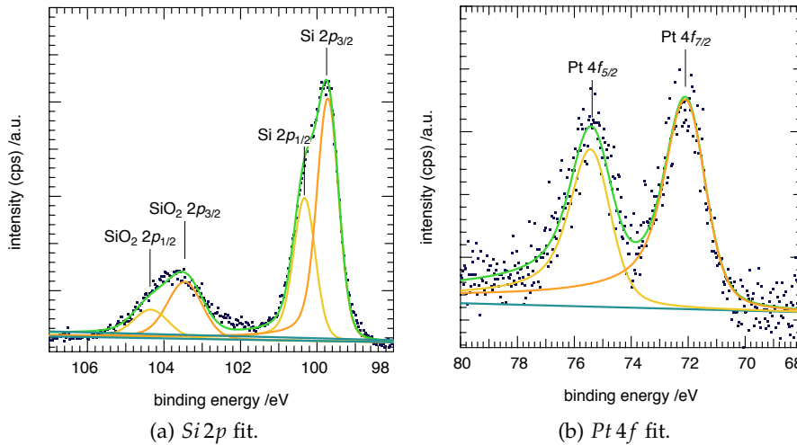
Figure 5.1.8: Representative Si\ 2p and Pt\ 4f peak and corresponding fits for 0.029\ e/nm^2\ Pt_{68} supported on a Si wafer. The results of the presented fits, for each position of the line scan are used to calculate the spatial distribution of clusters in fig. 5.1.10b.
