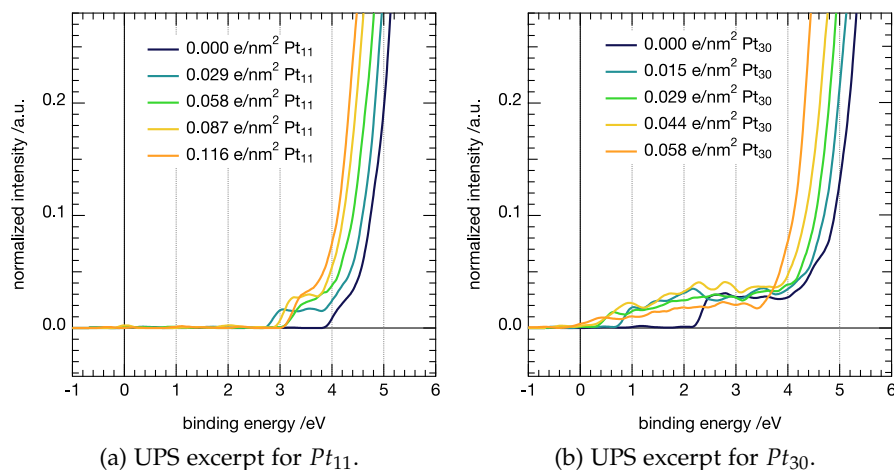
Figure 4.2.3: Excerpt of the normalized UPS spectra for better visibility in the region of the E_F as a function of Pt_{11} (a) and Pt_{30} (b) coverage.
