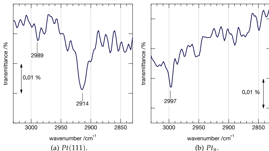
Figure 4.4.29: IRRAS of 0.4 \text{ C}_2\text{H}_4/\text{SA} adsorbed \text{C}_2\text{H}_4 on Pt (111) (a) and 0.203 \text{ e/nm}^2 \text{Pt}_n (b). The molecule was adsorbed at 100 \text{ K} .
