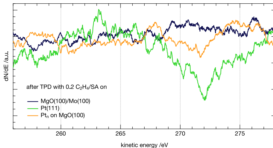
Figure 4.4.28: Excerpt of Auger electron spectra of the energy range between 255 – 278 eV after ethene desorption on MgO(100)/Mo(100) , Pt(111) and 0.203 e/nm^2 Pt_n on MgO(100) excited with an electron energy of 3 kV. The characteristic carbon peak C(KLL) at 272 eV is present for both the Pt single crystal, as the unselected clusters, however is not present for the support film MgO(100) [315, 333].
