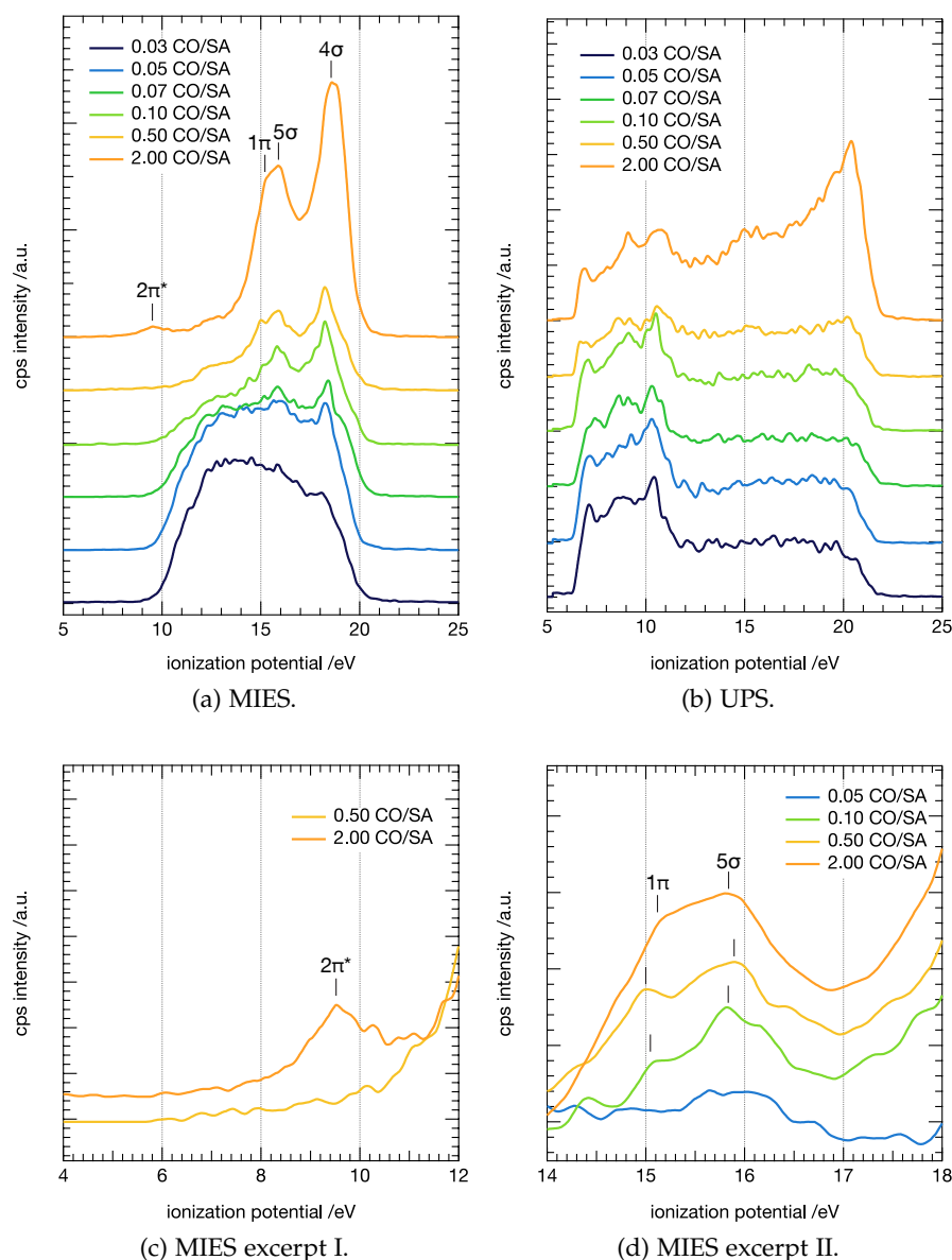
Figure 4.3.2: EES spectra of different amounts of CO adsorbed on Pt(111) - MIES (a) and UPS (b). Subfigures (c) and (d) show excerpts of the MIE spectra of selected coverages for better visibility of the CO peak features. For assignment of the CO MOs see text.
