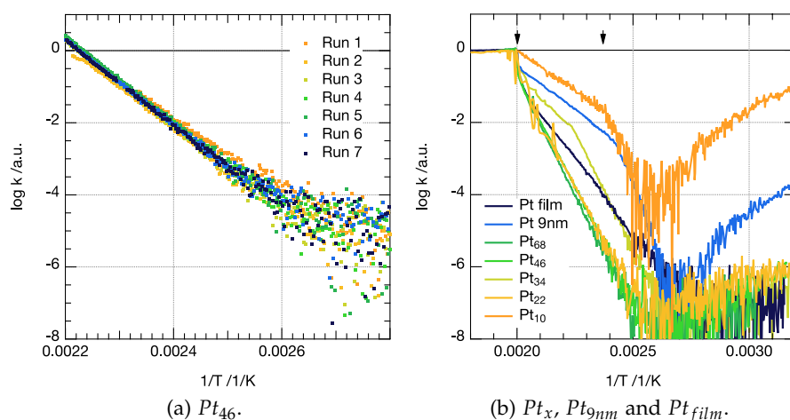
Figure 5.3.5: Arrhenius plots for the reactivity measurements shown in 5.3.3 for Pt_{46} , Pt_x , Pt_{9nm} and Pt_{film} . Arrhenius plots of different runs with increasing T for Pt_{46} (a) and for the highest reactivity of Pt_x , Pt_{9nm} and Pt_{film} (b). For better comparability all curves have been shifted to the same origin (a,b) and two arrows indicate the region used for the fit (b).
