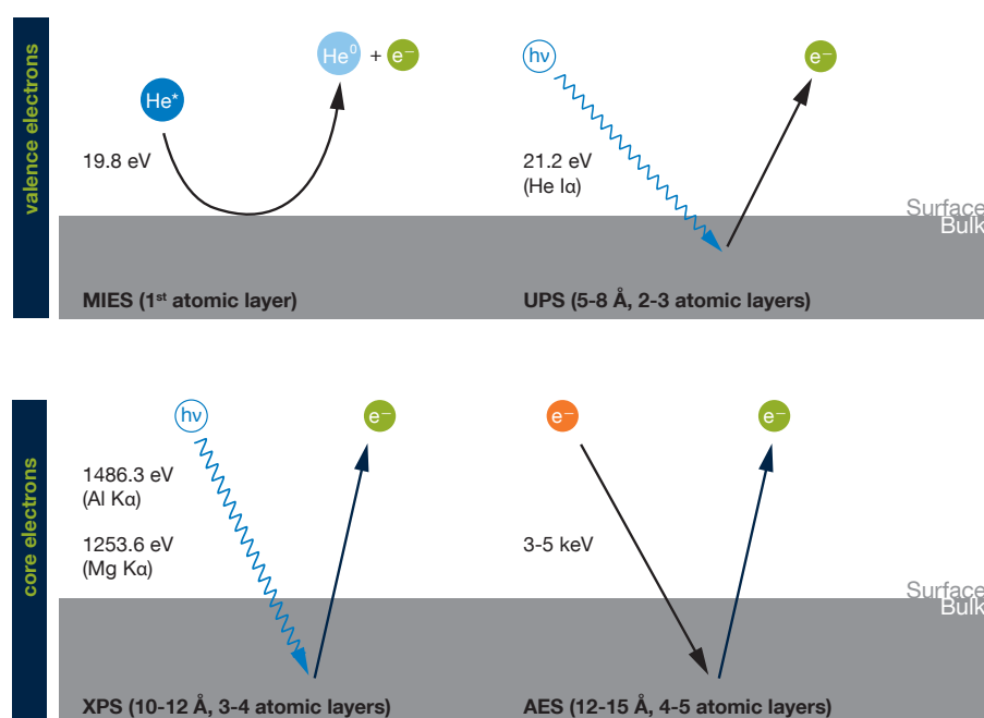
Figure 3.2.1: Summary of the EES used in this work: probe particle, corresponding excitation energies and surface sensitivity.
