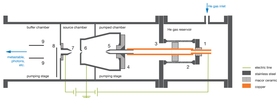
Figure A.1.4: Scheme of the utilized MIES/UPS setup: (1) Drilled current feedthrough, (2) bellow, (3) sandwich flange, (4) macror insulator, (5) cathode, (6) anode plate, (7) skimmer, anode for the second discharge, (8) chopper, and (9) deflector plates [213, 314]. Reprinted with permission from [314] - Copyright 2012, American Institute of Physics.
