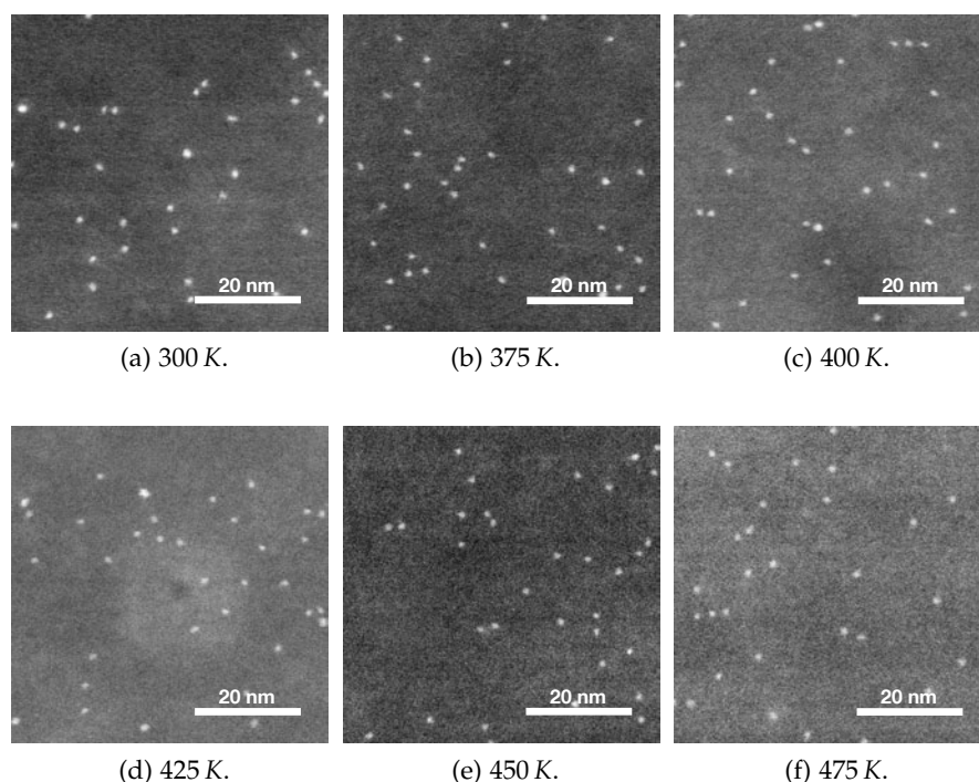
Figure 5.2.1: Excerpts ( 60 \times 60 \text{ nm}^2 ) of size-selected \text{Pt}_{46} clusters deposited onto 8 \text{ nm SiO}_2 at a coverage of 0.01 \text{ e/nm}^2 . The samples are probed under UHV conditions at the temperatures indicated.
