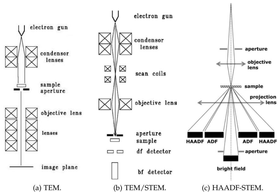
Figure 3.3.3: Schematic set-up of an electron microscope in the transmission (TEM) (a) and combined (TEM and STEM) (b) modes. Note how the dark field detector is off the central axis, as the dark field image is based on scattered electrons. The HAADF-STEM operation mode with bright- (on the central axis) and dark-field detectors (of the central axis) is shown in (c). Two different modes are available for dark field imaging, i.e. annular dark field (ADF); high-angle annular dark field (HAADF). Figures modified after [41].
