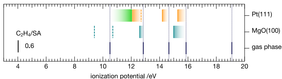
Figure 4.4.23: Shifts of the peak energy positions in MIES of the adsorbed C_2H_4 on MgO(100) and Pt(111) with respect to the peak positions of the gas phase spectra of Kimura et al. [143]. The orange and turquoise gradients represent relaxation shifts, the green gradient the possible chemical bond induced shift of peak I ( \pi_{C=C} ) on Pt(111) .
