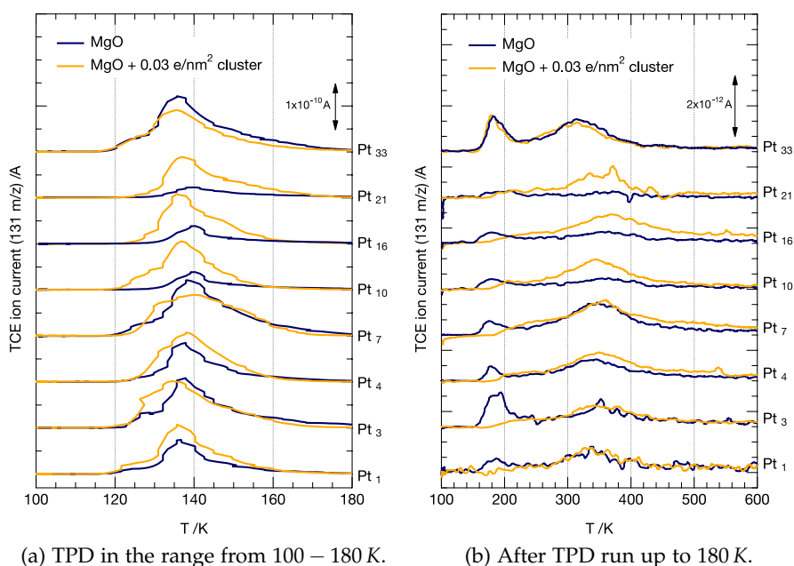
Figure 4.4.13: TPD spectra of 0.1 \text{ TCE}/\text{SA} adsorbed TCE on supported Pt_x clusters on \text{MgO}(100)/\text{Mo}(100) . Two different temperature ranges, TPD from 100 – 180 K (a) and subsequent TPD from 100 – 600 K (b) as well as TPDs from the pristine support (blue) and TPDs after deposition of 0.03 \text{ e}/\text{nm}^2 Pt_x (yellow) are shown. Note different scales for temperature and ion current.
