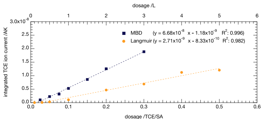
Figure A.1.2: Comparison of conventional Langmuir dosage ( L ) and the dosage by means of the molecular beam doser (MBD). Different dosage amounts of TCE on Pt(111) have been performed, followed by subsequent TPDs. The obtained TPD peaks have been integrated and plotted vs. the dosed amount. The single data points have been approximated by a linear fit. modified after [316].
