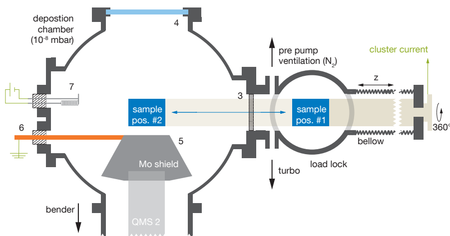
Figure 3.3.1: Sample preparation setup consisting of a rotary, linear stainless z-slide transfer manipulator attached to a UHV chamber cross. On the manipulator tip customized sample holders are fixed and can be moved between the positions (#1 and #2). The samples are prepared in a load lock, equipped with a differentially pumping system and separated by means of a pneumatic vacuum gate; for details see text.
