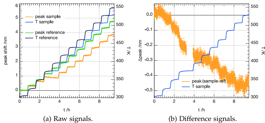
Figure 5.2.3: Plasmon change for stepwise heating (in 15\text{ K} steps, with 45\text{ min} for each temperature) of a Pt_{n \geq 53} sample and a corresponding reference sample (a) in Ar . A longer step at \sim 400\text{ K} for the sample and the corresponding temperature is caused by a fail in the heating. Difference signal, obtained by correction the sample signal for the temperature influence obtained from the reference sample (b).
