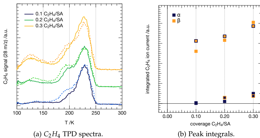
Figure 4.4.17: TPD spectra of ethene desorption on Pt(111) (a) with and without cleaning by means of sputtering in between. The dashed lines show the repetition experiment to the first TPD run on the clean surface. Three different coverages were studied and the corresponding peak integral values are plotted in (b), the points with border represent the corresponding second runs.
