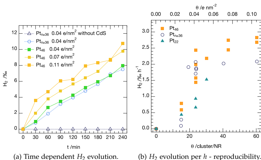
Figure 5.4.5: H_2 evolution as a function of time for representative samples (a) and for all coverage dependent measurements as H_2 evolution per hour (b). In fig (a) the hydrogen generation as function of time for unselected Pt_{n \geq 36} (open circle) and selected Pt_{46} (filled squares) clusters deposited on CdS NRs or on blank support (open triangles) are shown. Each point represents the total amount of hydrogen produced by the sample at that time. The sample without NR shows no photocatalytic activity, whereas all other samples show a linear trend over time. Fig (b) shows the hydrogen generation per hour (after four hours of illumination) for Pt_{n \geq 36} , Pt_{22} and Pt_{46} . The observed variations demonstrate a highly reproducible measurement and sample preparation procedure. A smooth trend with increasing coverage and reaching of a saturation level (for Pt_{n \geq 36} and Pt_{46} ) can be seen. Reprinted (adapted) with permission from [220] - Copyright (2012) American Chemical Society.
