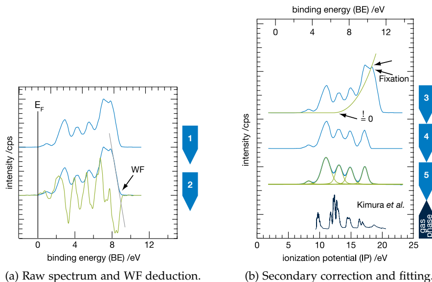
Figure A.1.5: Post detection data treatment steps applied for MIE/UP spectra of adsorbed molecules, exemplarily shown for for 0.125 TCE/SA on Mo(112). Raw spectrum (1), WF determination with differentiated spectrum and tangent (2). Shift from BE (a) to IP (b). Secondary electron background correction by subtracting a fitted polynomial function (3), background corrected spectrum (4), fitted spectrum and sum curve (5); gas phase spectrum on the bottom. Roman numerals on top of the bottom spectra assign the peaks of the corresponding gas phase EES spectra [143]. Reprinted (adapted) with permission from [172] - Copyright (2012) Elsevier.
