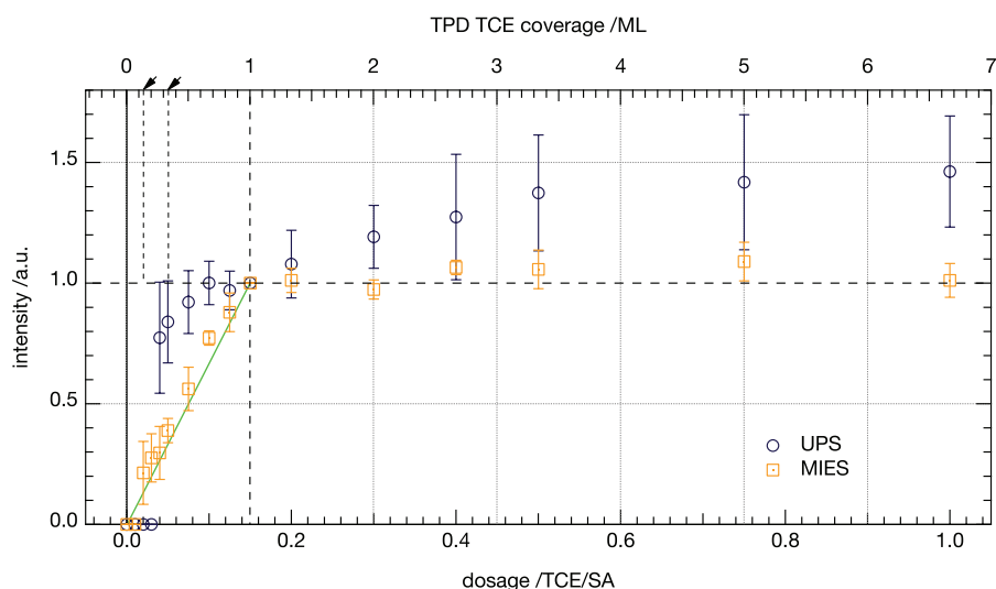
Figure 4.1.1: Representative MIES/UPS peak intensities for TCE on Mo (112) plotted against the dosed amounts of TCE (bottom) and the corresponding coverage in ML (top) as determined from TPD. For each data point the peak intensities of the peaks I to IV have been averaged and normalized to the filled first ML (completion of the physisorbed layer in TPD, dashed line). The errors of the data points are the standard deviation of the four averaged peak intensities. For MIES data a saturation of the peak intensity is visible for a filled first ML , whereas for UPS the intensities increase up to a coverage of four ML corresponding well to the expected probe depth of the method. The arrows indicate 1/6 ML and 1/3 ML . Reprinted (adapted) with permission from [172] - Copyright (2012) Elsevier.
