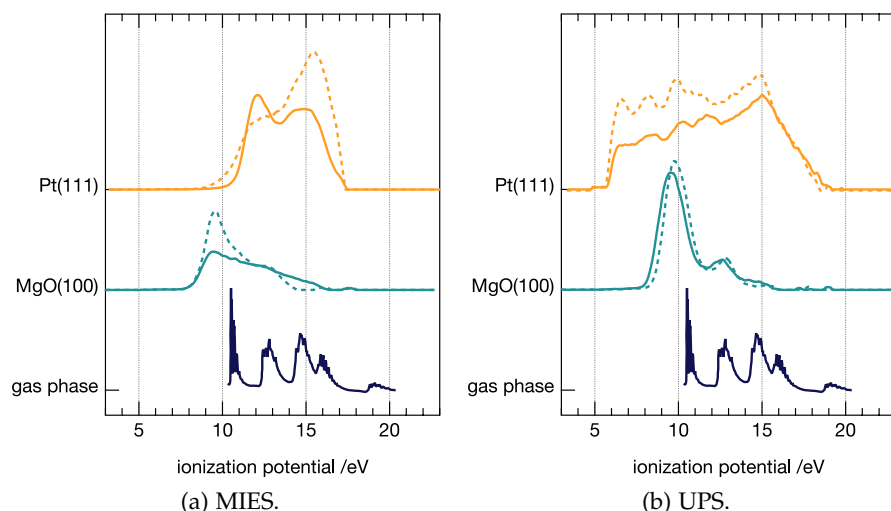
Figure 4.4.22: EE spectra of 0.6 C_2H_4/SA on MgO(100) and Pt(111) , for comparison the pristine surface spectra are shown in dashed lines in the same colour. From bottom to top: gas phase spectrum from Kimura et al. [143] and MgO(100)/Mo(100) and Pt(111) on IP energy scale; MIES (a) and UPS (b).
