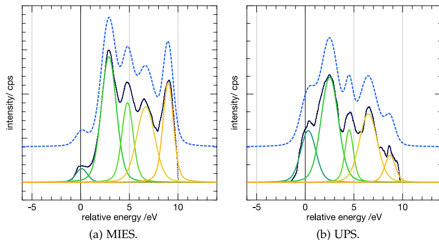
Figure 4.4.4: EES spectra (MIES (a), UPS (b) - dark blue) for 0.5 TCE/SA on MgO(100) and the corresponding fit functions (green to yellow) for the five TCE features, as well as the corresponding sum of the fit functions (dashed light blue).
