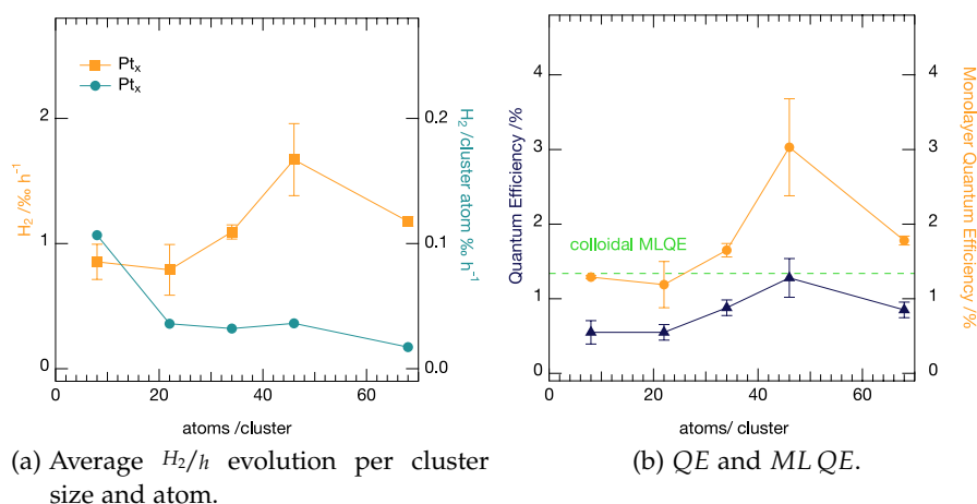
Figure 5.4.8: H_2 production per hour (after four hours of illumination) (a) and (ML) QE (b) for selected Pt_x ( x = 8, 22, 34, 46, 68 ) decorated photo catalysts as a function of cluster size at a coverage of 0.04 e/nm^2 . In (a) the data points represent the averaged multiple measurements, as shown in fig. 5.4.7b. Error bars shown, are based on the standard deviation of multiple measurements per cluster size - the lines connecting the data points serve as a guide to the eye. Hydrogen production per hour (orange squares, left axis) shows a maximum for Pt_{46} , whereas larger as well as smaller sizes reveal lower hydrogen yields. Hydrogen production per single cluster atom (green circles, right axis) shows a maximum hydrogen evolution for Pt_8 decorated samples and decreases with increasing cluster size. A similar trend as for the H_2/h production is displayed for (ML) QEs (b). For comparison, the saturation ML QEs for the colloidal Pt/CdS NRs (green dashed line) photocatalyst system is included.
