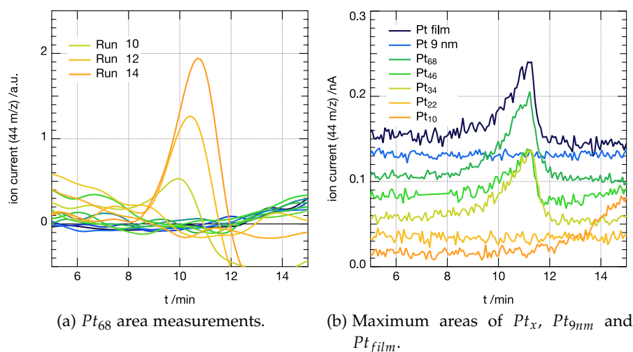
Figure 5.3.2: Area measurements of Pt_{68} during a measurement up to 453 K, only the runs 10, 12, 14 show a signal (smoothed) and are labeled in the legend (a). Representative maximum areas, after measurement (up to 453 K), for different sizes along with larger particles and the thin film (b).
