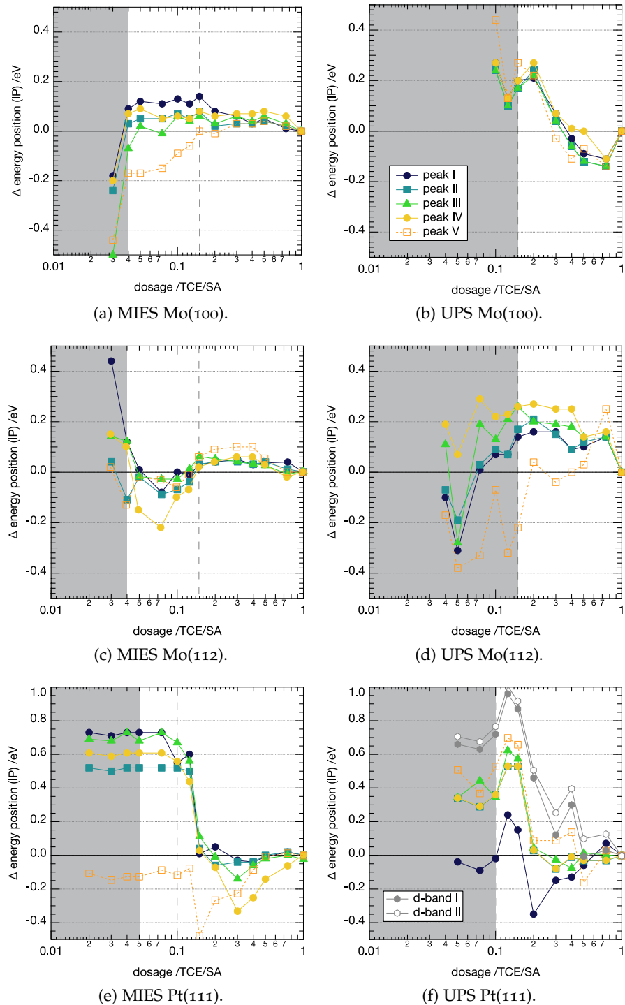
Figure 4.4.11: Shifts of the peak energy positions in EES of the TCE MOs on the studied surfaces. The dosed amounts are plotted in log scale for better visibility of the submonolayer range. Corresponding ML (dashed line) and range in which not all peaks are visible in accordance with the values from tab. 4.4.1 (gray areas). The relative energies are plotted with respect to the position at the final coverage of 1 TCE/SA. Peak V is plotted in dashed lines, as systematic errors seem introduced by the background fitting procedure. The error of these data is apparent from the data scatter. Reprinted (adapted) with permission from [172] - Copyright (2012) Elsevier.
