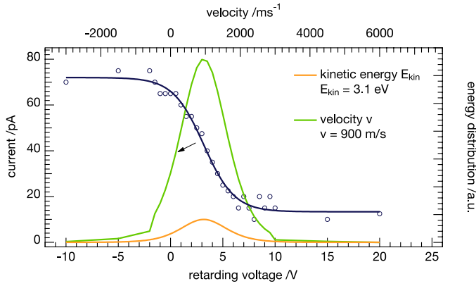
Figure 3.1.3: Retarding field analysis for size-selected Pt_{11}^+ clusters deposited in the UHV chamber; measured current (blue) as a function of the retarding potential, the kinetic energy (derivative, orange) and the velocity distribution (green).
