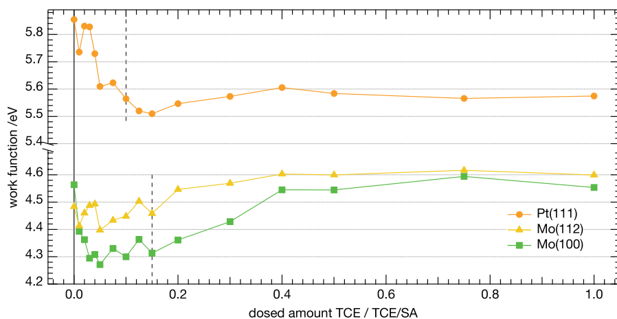
Figure 4.4.9: WF with increasing coverage of TCE on the studied surfaces. The values are determined from the corresponding UPS measurements; the dashed lines represent the corresponding ML determined by TPD measurements. The values have a statistical error of \pm 0.05 eV, for details see text. Reprinted (adapted) with permission from [172] - Copyright (2012) Elsevier.
