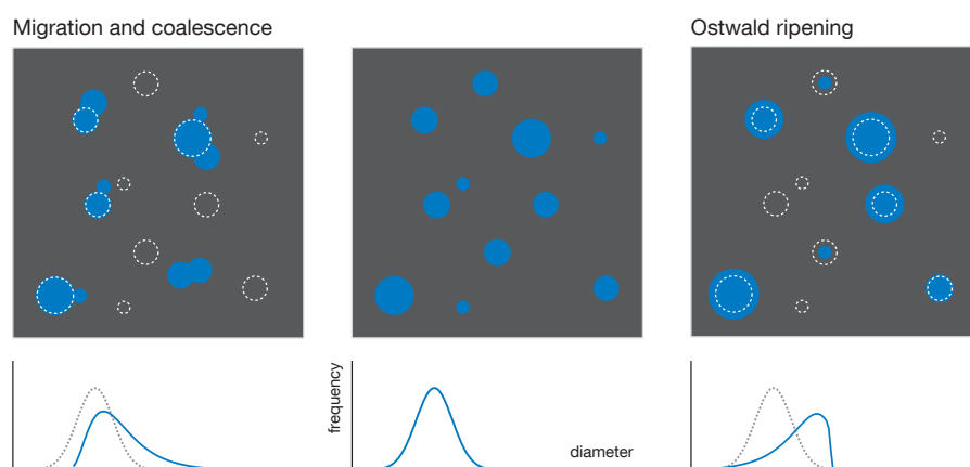
Figure 2.3.1: Schematic illustration of Ostwald ripening (right) and Migration and coalescence (left) sintering processes of particles on surfaces. Below are shown the corresponding, theoretically to expect PSD.
