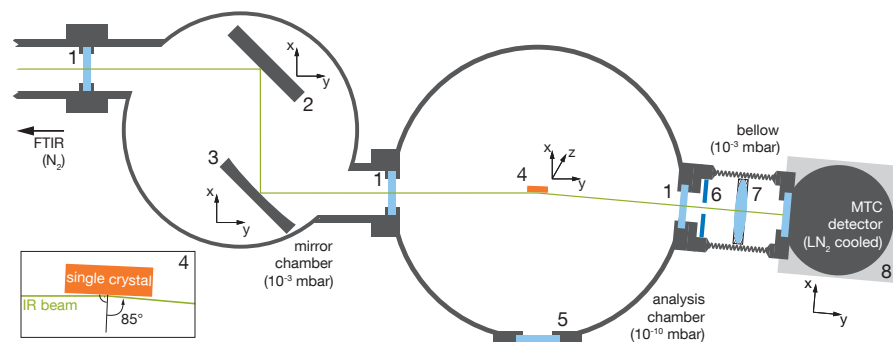
Figure 3.2.7: Top view of the IRRAS setup in the nanocat lab, the insert (left bottom corner) shows the passing IR beam at a glazing angle of 85^\circ , with respect to the surface normal of the single crystal (4). For details see text.
