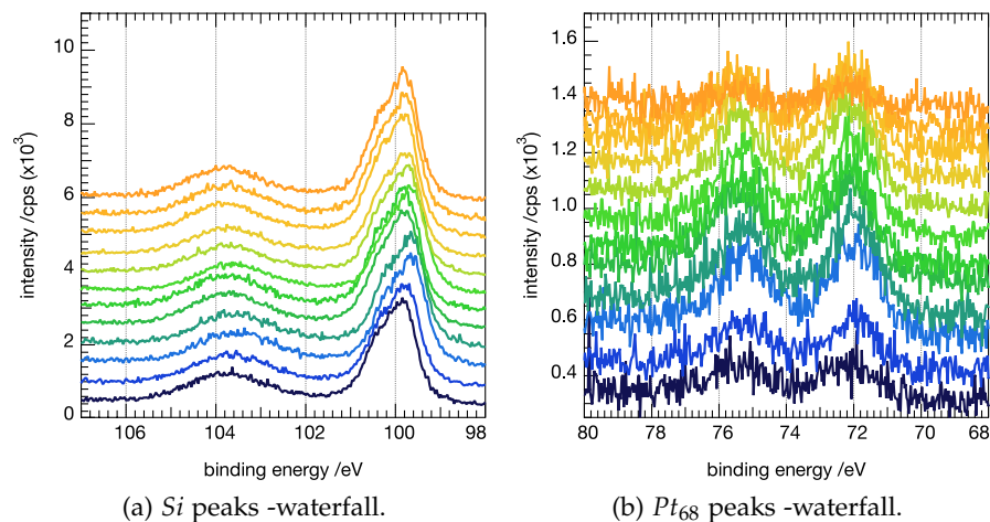
Figure 5.1.9: XPS line scan excerpts of the Si 2p (a) and Pt 4f (b) peaks for the sample with 0.029 e/nm^2 Pt_{68} supported on a Si wafer. The obtained fit results of these signals (i.e. Pt in fig. ) are used to calculate the spatial distribution of clusters in fig. 5.1.10b.
