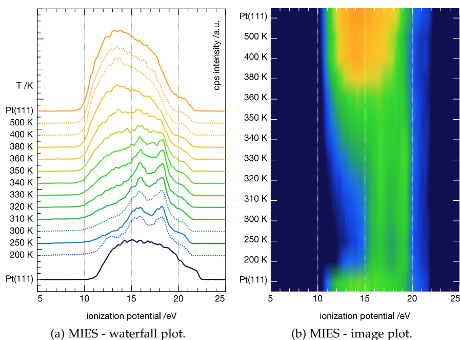
Figure 4.3.4: MIE spectra of CO desorption after stepwise heating on Pt(111) . On the surface 0.4^{CO/SA} are adsorbed at 100 K , the crystal is then heated in several steps and cooled down before each MIE spectra. The desorption reveals the support features after 360 K - MIES raw spectra (a) and image plot (b).
