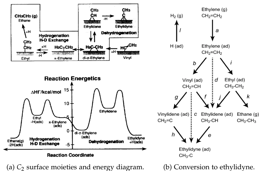
Figure 2.1.1: Reaction scheme and energy diagram for the surface chemistry occurring during thermal conversion of ethene via hydrogenation on Pt (111) (a). The mechanisms shown, for both the conversion of ethene to ethylidyne (via an ethylidene intermediate) and for H – D exchange and hydrogenation reactions (via a common ethyl moiety) [62]. Possible reaction pathways for ethylidyne formation over Pt group metals at T > 200 K, (b), three mechanisms are suggested: mechanism 1 (a,b,f and e), mechanism 2 (a,b,g and h) and mechanism 3 (a,i,j and e) [111].
