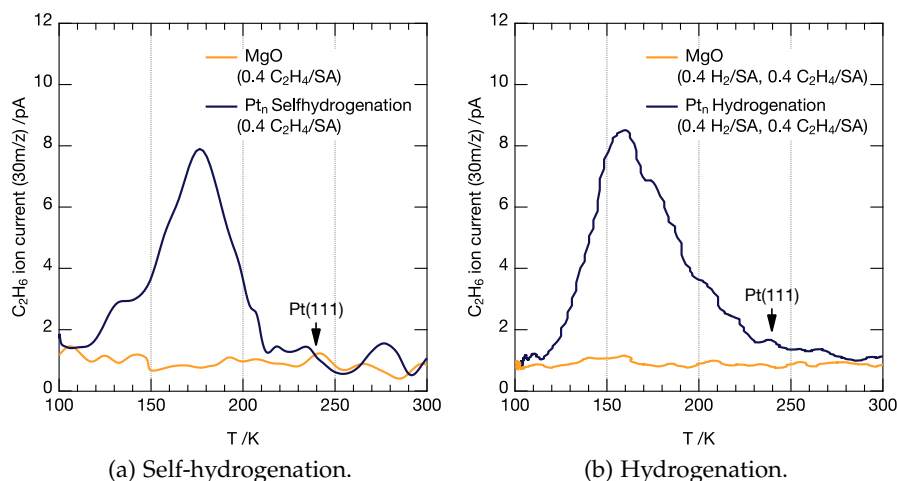
Figure 4.4.26: TPR spectra ( \beta = 2K/s ) of self-hydrogenation (a) and hydrogenation (b) of ethene on 0.203 e/nm^2 unselected Pt_n clusters (blue spectra). The previous taken TPR on the corresponding pristine MgO supports is additionally shown (orange spectra), however reveal no reactivity. An arrow indicates the position of the peak maximum for the experiment on the Pt(111) for comparison.
