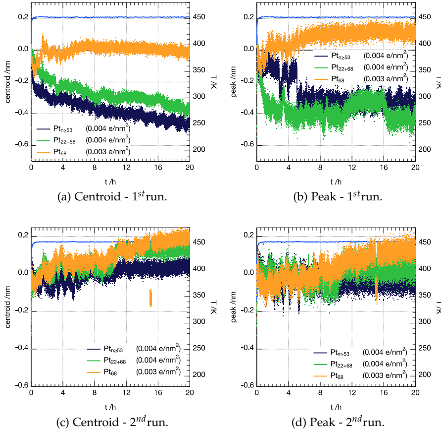
Figure 5.2.4: INPS signals of Pt_{x,n} ( x=68, 68+22, n \geq 53 ) at 453 K under Ar atmosphere, centroid signal (left) and peak shift (right) for two annealing cycles ( 1^{st} run top, 2^{nd} run bottom).
