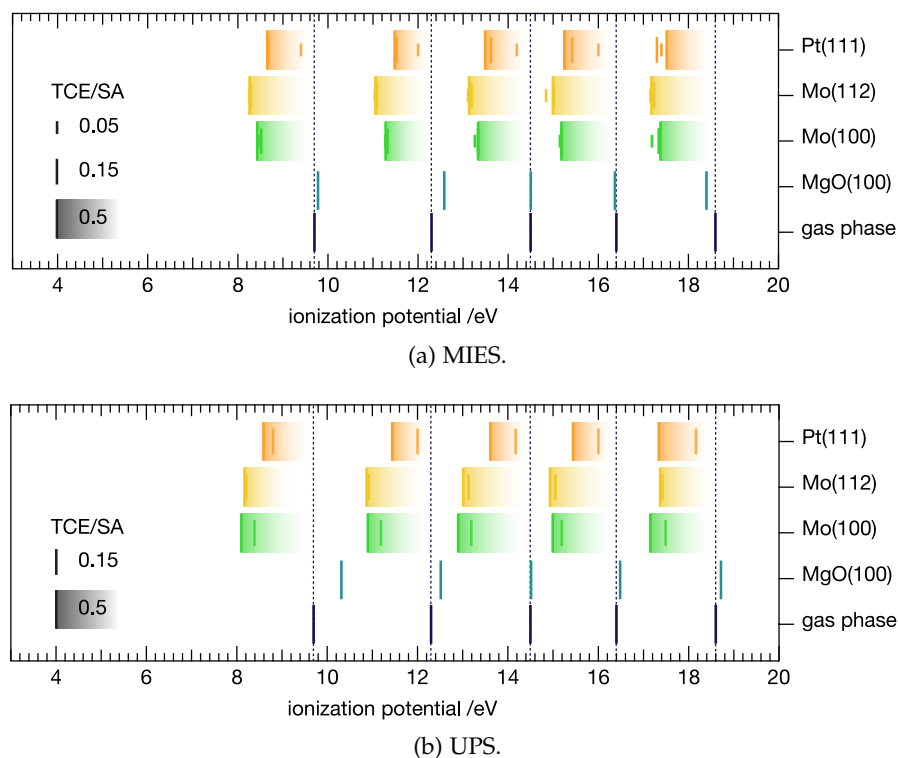
Figure 4.4.10: Shifts of peak energy positions on the various surfaces with respect to the peak positions of the gas phase spectra of Kimura et al. [143]; MIES (a) and UPS (b). For MIES three selected coverages, for UPS two coverages (above the ML ) are shown. The height of the lines reflect the dosed TCE concentrations on the surface: 0.05 (MIES only), 0.15 and 0.5 TCE/SA , corresponding to physisorbed species only, filled first ML and physisorption with condensation on top, respectively. Due to charging of the MgO substrate (see text) only the peaks for the highest TCE coverage are shown with the energy position of peak II aligned to the one of the gas phase spectrum. Reprinted (adapted) with permission from [172] - Copyright (2012) Elsevier.
