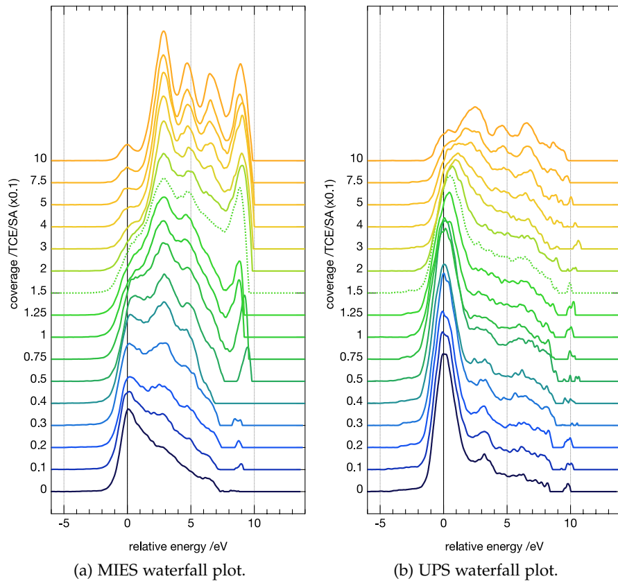
Figure 4.4.3: EE spectra of adsorbed TCE on MgO(100) , referenced on the first peak (relative energy E_R = \text{zero} ) and background corrected. The plot shows increasing dosage of TCE from bottom to top. The bottom spectra show the clean MgO(100) surface; the dashed line indicates the saturation of the first ML, determined from TPD measurements. Reprinted (adapted) with permission from [172] - Copyright (2012) Elsevier.
