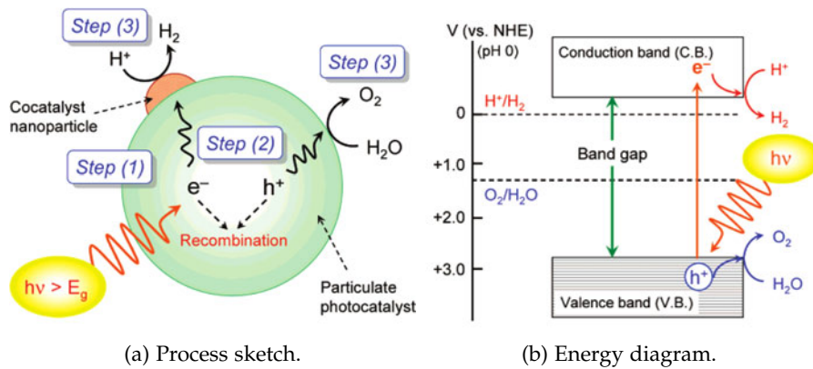
Figure 2.1.2: Illustration of the mechanism of photocatalytic water splitting and corresponding energy diagram. The process (a) involves three steps: photon absorption generating electron-hole pairs (step 1), charge-carrier separation (and recombination, step 2) and surface reduction/oxidation reactions (step 3). Schematic energy diagram (b) for exciton mediated water -splitting in a semiconductor. A minimum band gap size of 1.23 V vs. NHE and suitable band edge positions are prerequisite [69].
