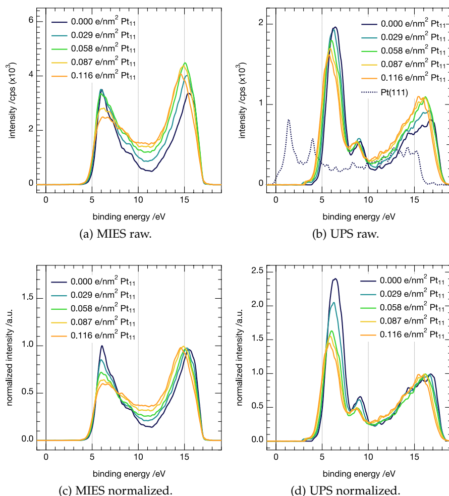
Figure 4.2.1: EES of four different Pt_{11} coverages on MgO support. Raw spectra (top) as well as normalized spectra with respect to the peak of the secondary electron emission (bottom) are shown. MIES (left) and UPS (right) are plotted on an BE scale. The maximum coverage of 0.116 e/nm^2 corresponds to a coverage of 0.5 \%ML . For (b) the Pt(111) spectra is shown for comparison.
