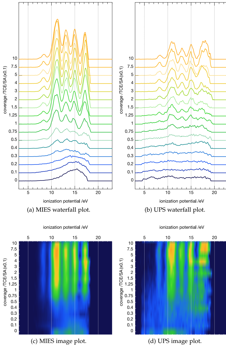
Figure 4.4.6: EE spectra of adsorbed TCE on Mo(112) , referenced with respect to the vacuum level of the clean substrate and background corrected. Increasing dosage of TCE from bottom to top; MIES (a) and UPS (b). The bottom spectra show the clean Mo(112) surface. The dashed lines indicate the coverages (0.05, 0.15 and 0.5 TCE/SA) for which the IP energy shift is shown in fig. 4.4.10. Subfigures (c) and (d), show the corresponding image plots for better visibility of the appearance of the TCE peak features for MIES and UPS, respectively. Reprinted (adapted) with permission from [172] - Copyright (2012) Elsevier.
