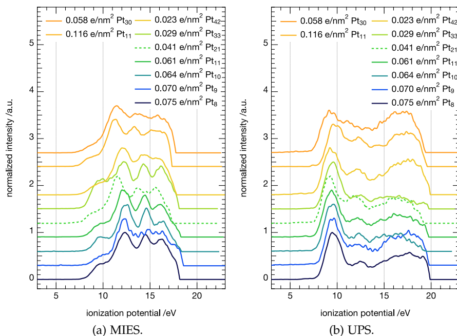
Figure 4.4.14: EE spectra of 0.1 TCE/SA adsorbed TCE on supported Pt_x clusters on MgO(100)/Mo(100) , referenced with respect to the vacuum level by addition of a fixed WF value of 3.5 eV of the clean support ( MgO ) and background corrected. Increasing Pt_x cluster size from bottom to top; MIES (a) and UPS (b). The dashed line indicates a not trustworthy spectra of Pt_{21} .
