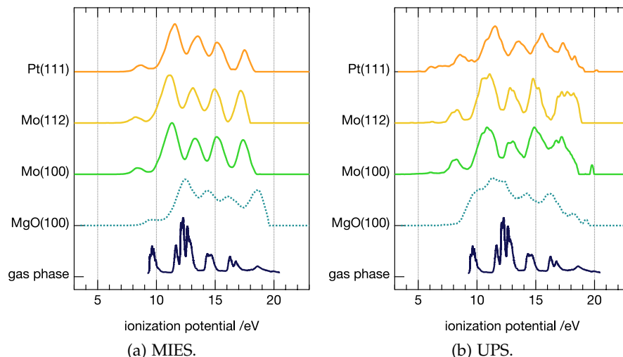
Figure 4.4.8: EE spectra of 0.5 TCE/SA (equal to physisorbed and multilayer TCE ) for the investigated surfaces. From bottom to top: gas phase PE spectrum from Kimura et al. [143] and MgO(100)/Mo(100) displayed for comparison (aligned to the gas phase spectra, by adding the gas phase value of the TCE peak I with 9.7\text{ eV} to the arbitrary origin on the relative energy scale at the first O2p feature of the MgO support, see text); Mo(100) , Mo(112) and Pt(111) on IP energy scale; MIES (a) and UPS (b). Reprinted (adapted) with permission from [172] - Copyright (2012) Elsevier.
