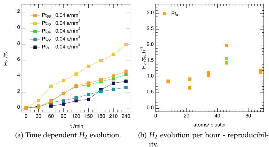
Figure 5.4.7: H_2 evolution as a function of time for representative samples of the different sizes (a) and the result of all coverage dependent measurements as H_2 evolution per hour (b). In fig. (a) the hydrogen generation as function of time for representative samples with the sizes Pt_x ( x = 8, 22, 34, 46, 68 ) deposited on CdS NRs are shown. Each point represents the total amount of hydrogen produced by the sample at that time; all samples reveal a linear trend over time, with a slope dependent on the size. Fig. (b) shows the hydrogen generation per hour (after four hours of illumination) for all measured samples and the observed small variations per size demonstrate high reproducibility.
