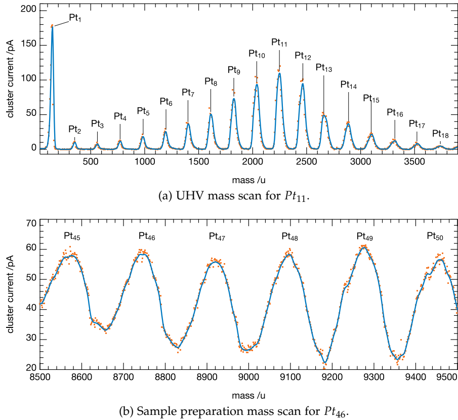
Figure 3.1.2: Different ranges of mass scans, showing the size distributions of Pt^+ clusters selected by the QMS for the UHV part (a) optimized for Pt_{11} and for the sample preparation (b) for Pt_{46} . The orange dots represent the raw data, which has been smoothed for better visibility of the trend (blue lines).
