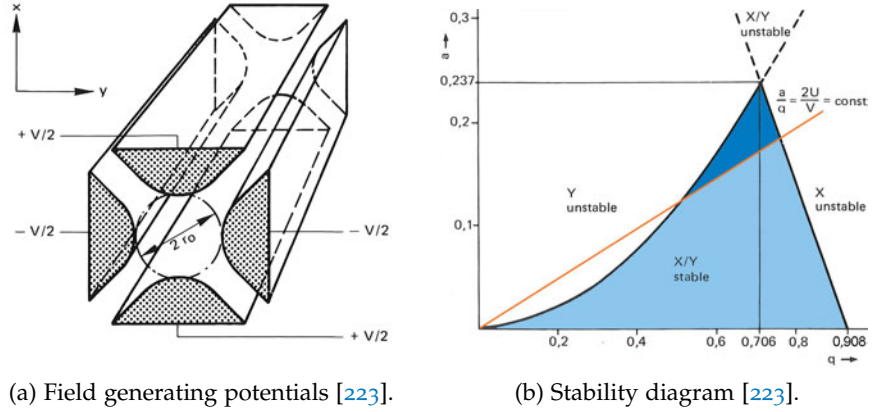
Figure 3.1.1: Field generating potentials (a) and stability diagram (Mathieu diagram) (b) of a QMS. The blue shaded areas represent values of a and q which give rise to bounded trajectories. The complete blue area defines the stability region for ions when passing through the QMS for RF-only conditions ( a = 0 ), however when applying an additional DC potential (in the plotted case the ratio a/q = 2U/V = \text{const.} ) only the dark blue area is stable, defined by the orange line - also known as the mass scan line.
