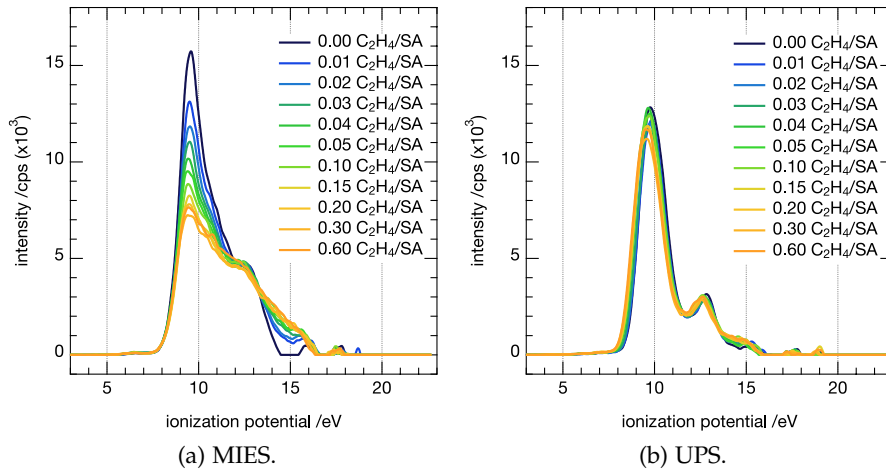
Figure 4.4.18: EE spectra of adsorbed C_2H_4 on MgO(100) as a function of coverage, referenced with respect to the vacuum level of the clean substrate and background corrected - MIES (a) and UPS (b).
