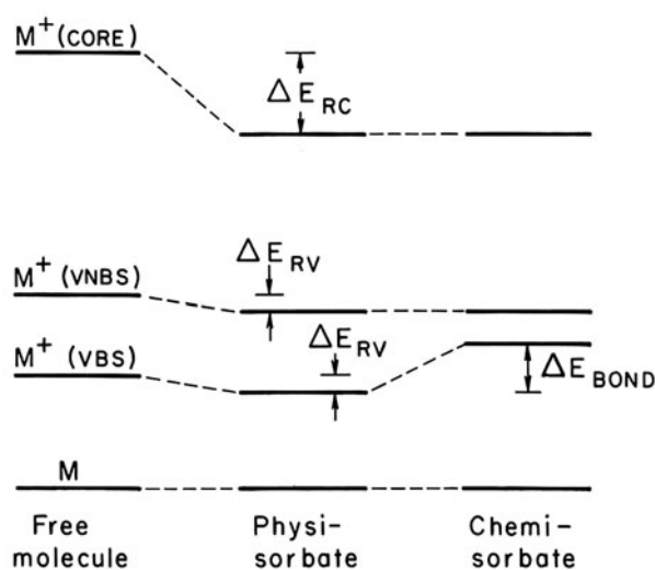
Figure 2.2.2: Energy level diagram for EES (on an IP scale) from an adsorbate molecule, showing ground state M , core-hole state M^+(\text{core}) , as well as hole states M^+(\text{VBS}) and M^+(\text{VNBS}) of binding and non-binding valence orbitals to the substrate, respectively. Hole-state energies (BE) are lowered ( \Delta E_{RV} ) upon physisorption, because of screening by the substrates (note the bigger relaxation for core holes \Delta E_{RC} ). Upon chemisorption, the bonding orbital can be identified by an increase \Delta E_{BOND} in BE, may however include contributions of \Delta E_{RV} [165].
