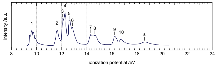
Figure A.3.5: Gas phase photo electron spectrum of trichloroethene adapted from [143].
