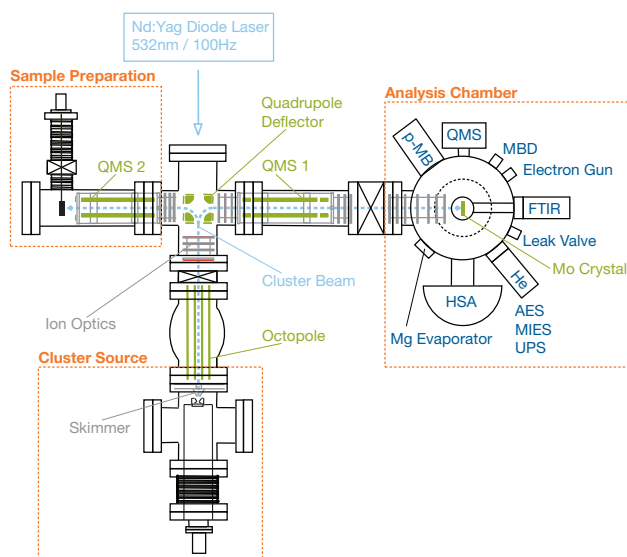
Figure 3.0.2: Schematic sketch of the nanocat experimental setup (top-view). The setup is divided into three major parts (boxes with dashed orange lines): cluster source (bottom), sample preparation (top left) and analysis chamber (top right) [17, 29, 213, 20, 38].
