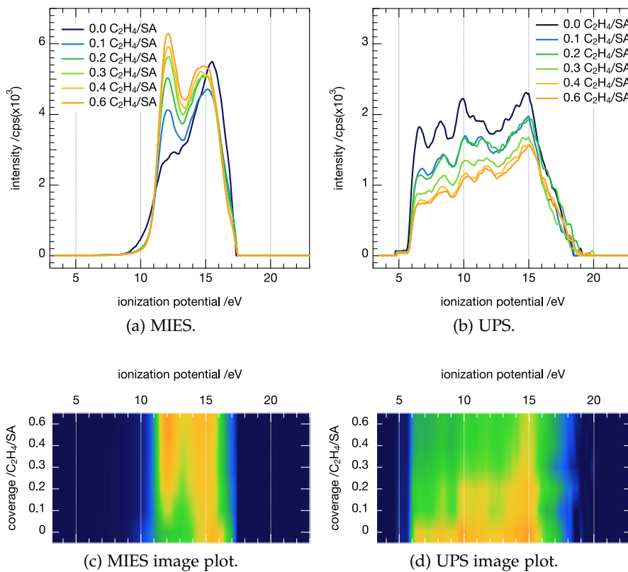
Figure 4.4.19: EE spectra of adsorbed C_2H_4 on Pt(111) as a function of coverage, referenced with respect to the vacuum level of the clean substrate and background corrected - MIES (a) and UPS (b). Subfigures (c) and (d), show the corresponding image plots for better visibility of the appearance of the C_2H_4 peak features for MIES and UPS, respectively.
