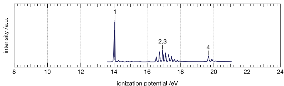
Figure A.3.1: Gas phase photo electron spectrum of carbon monoxide adapted from [143].
