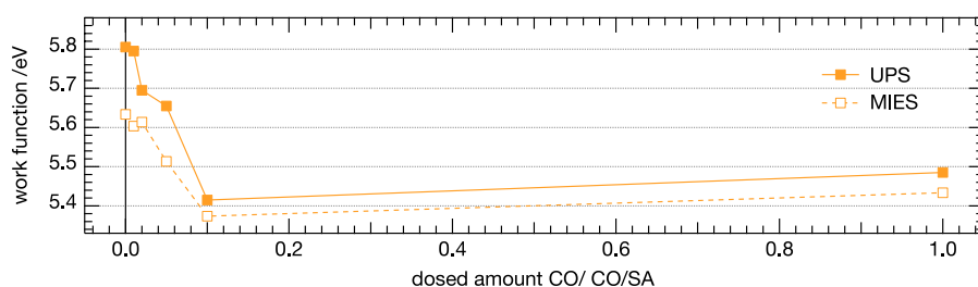
Figure 4.3.3: Absolute WF changes with increasing coverage of CO on Pt(111). The values are determined from the corresponding EES measurements and have a statistical error of \pm 0.05\text{ eV} .
