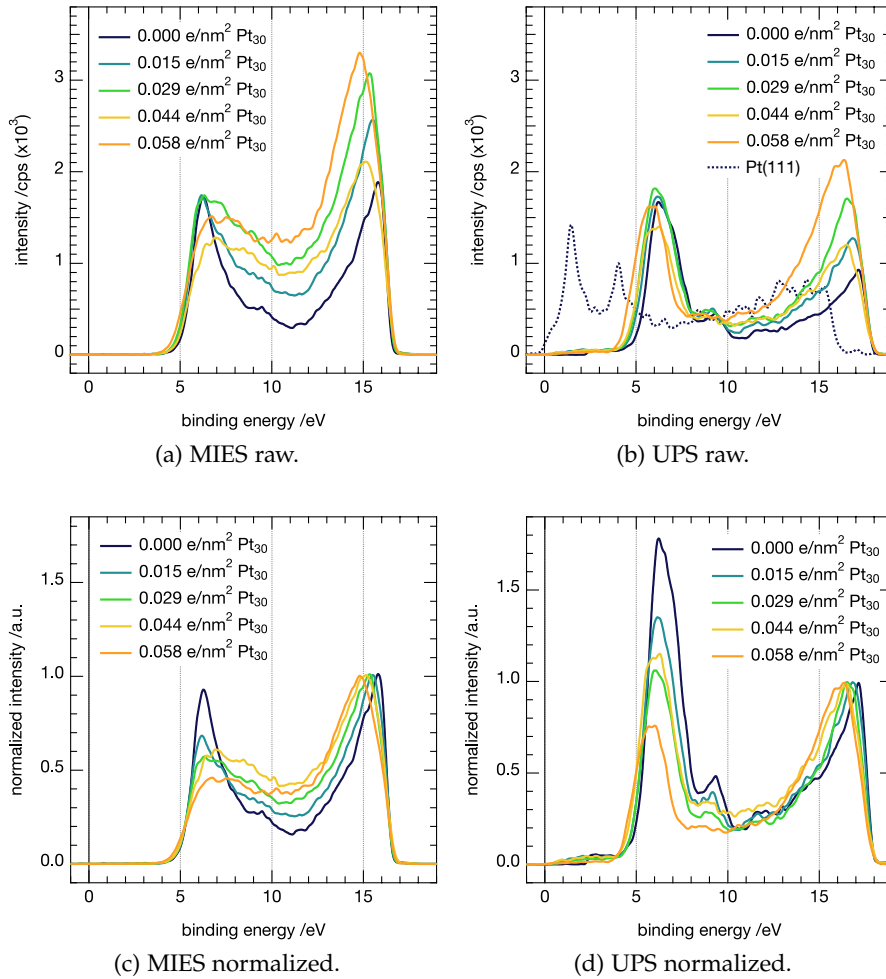
Figure 4.2.2: EES of different Pt_{30} coverages on MgO support. Raw spectra (top) as well as normalized spectra with respect to the peak corresponding to the emission of secondary electrons at the high binding energy cut off (bottom) are shown. MIES (left) and UPS (right) are plotted on an BE scale. The maximum coverage of 0.058 \text{ e/nm}^2 corresponds to a coverage of 0.2 \%ML . For (b) the Pt(111) spectra is shown for comparison.
