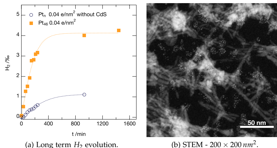
Figure 5.4.10: Results of long-term H_2 evolution measurements (a) and HAADF-STEM measurement after reaction (b). The long term measurement (a) on unselected and selected clusters is displayed as a function of time; the interpolation of the raw data points (dashed lines) serves as a guide to the eye. Deviations from the linear relation (after first 240 min) indicate catalyst deactivation; after about 400 min of measurement no further hydrogen evolution is observed. A corresponding micrograph (b) taken of a Pt_{46} sample after illumination and H_2 production over 25 h shows flocculated NRs as big white spots and groups of cluster ensembles in between. Single clusters have spatially approached but are not coalesced.
