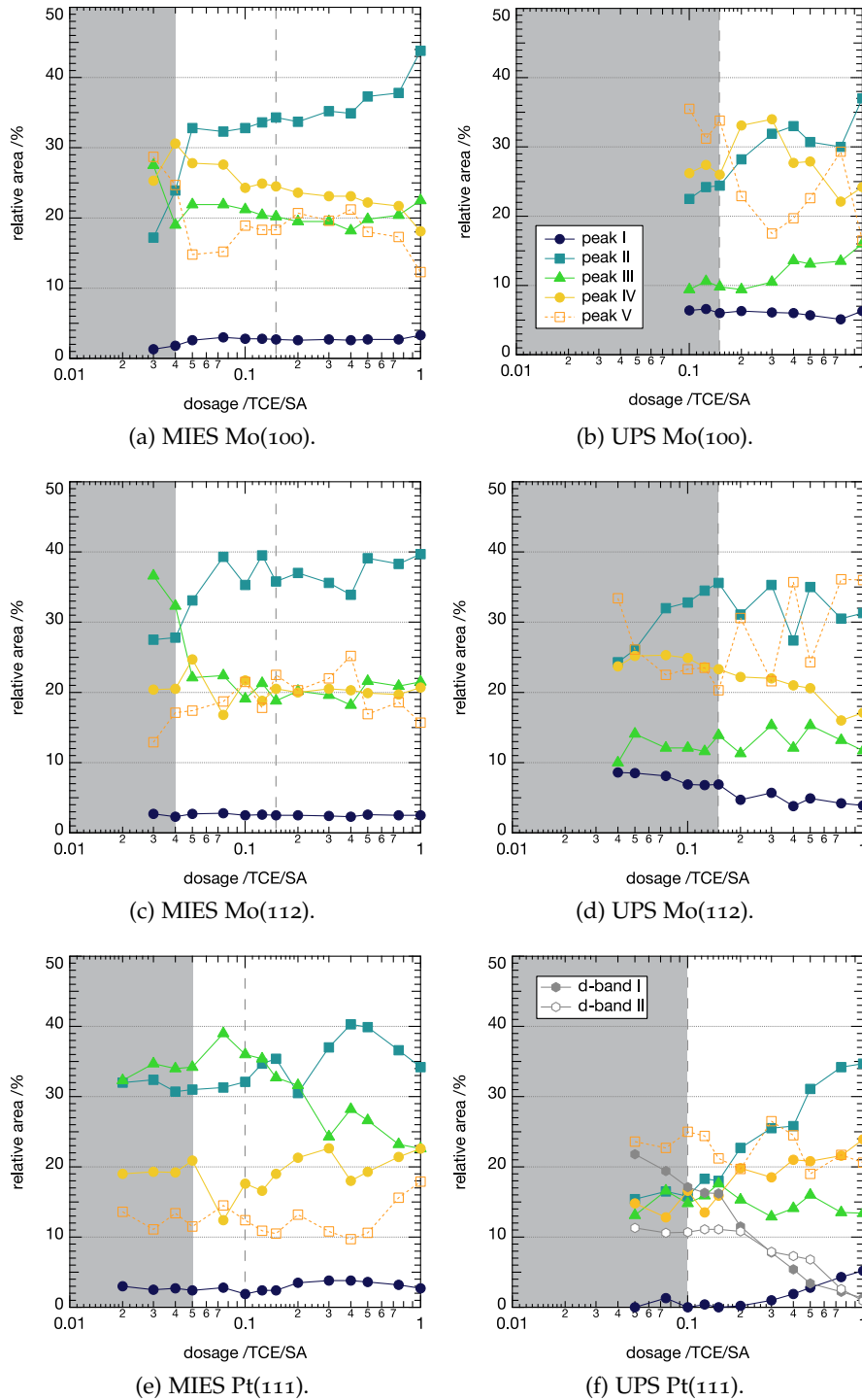
Figure 4.4.12: Changes in relative area for obtained from the fit values (peak I-IV) from 0.03 TCE/SA for MIES (a,c,e) and from 0.1 TCE/SA on for UPS (b,d,f). The dosed amounts are plotted in log scale for better visibility of the submonolayer range; corresponding ML marked with dashed line and gray area represents the range in which not all peaks are visible (tab. 4.4.1). For Pt the d -band peak positions are shown, peak V is plotted in dashed lines (systematic errors). The error of these data is apparent from the data scatter, for details see text. Reprinted (adapted) with permission from [172] - Copyright (2012) Elsevier.
