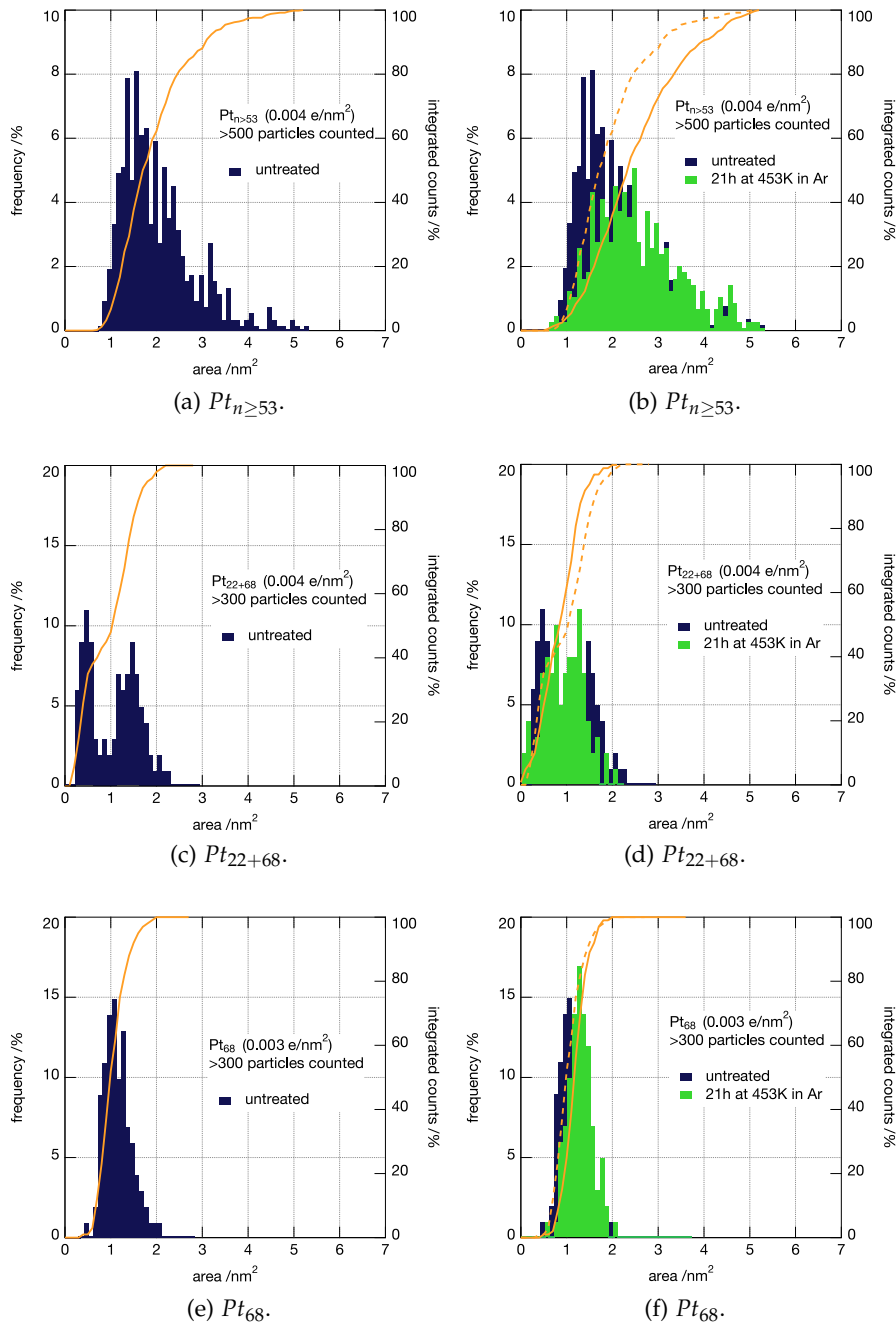
Figure 5.2.5: Corresponding ADF histograms to the TEM samples treated in a similar way as the INPS samples in fig. 5.2.4. The PSD on the left (a,c,e) represent the initial areas (blue) observed for the samples along with the integrated counts. The histograms on the right (b,d,f) show additionally the ADF for the samples heated to 453 K for 21 h under an Ar (green). For a better comparison, the PSD and integrations (dashed lines) of the initial state are shown as well. From top to bottom, Pt_{n>53} , Pt_{22+68} and Pt_{68} are depicted.
