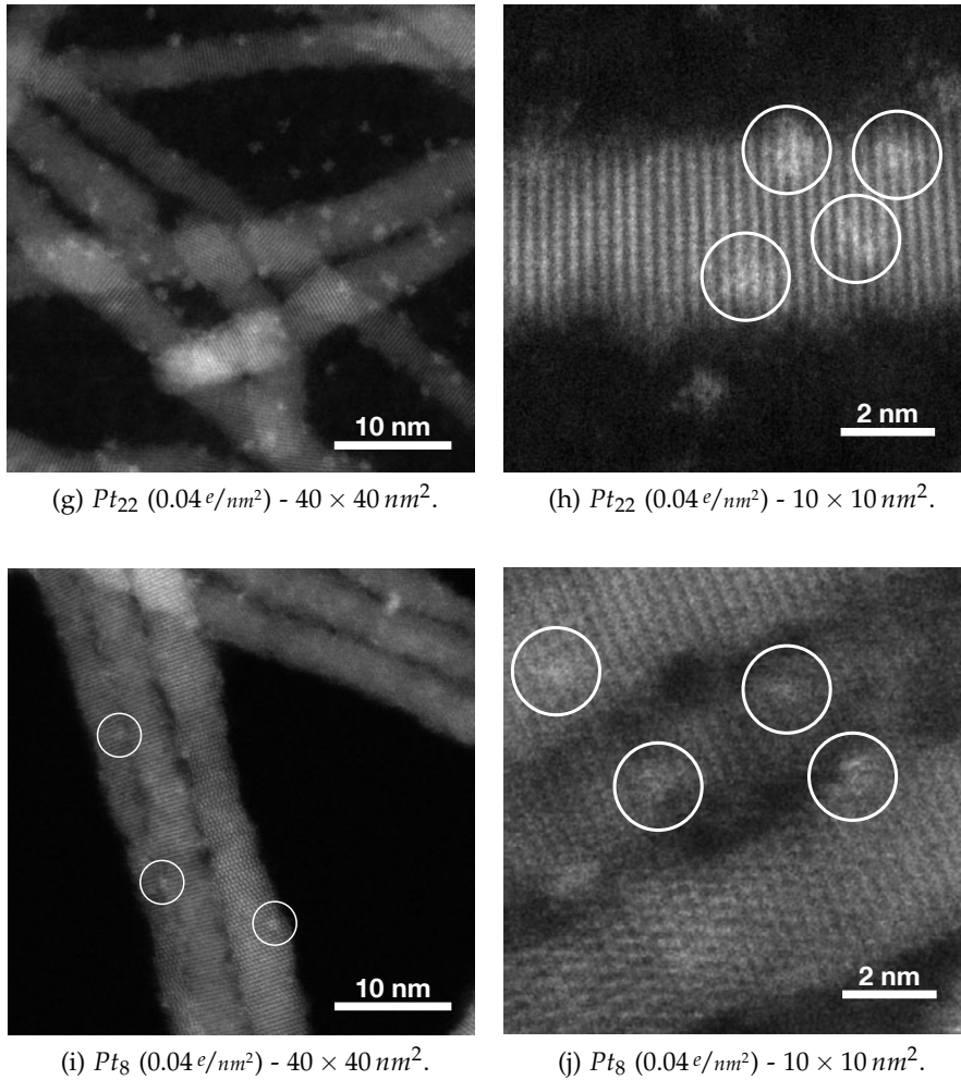
Figure 5.4.3: HAADF-STEM micrographs ( 40 \times 40 nm^2 and 10 \times 10 nm^2 ) of size-selected Pt_x ( x = 8, 22, 34, 46, 68 ) clusters deposited onto CdS NR thin films at a coverage of 0.04 e/nm^2 . The amount of clusters fit the expected values and for different sizes the cluster size in the image vary accordingly. Images at high magnification even allow for resolving atomic structure of rod and Pt clusters. For better visibility clusters in the 10 \times 10 nm^2 excerpts are marked by white circles.
