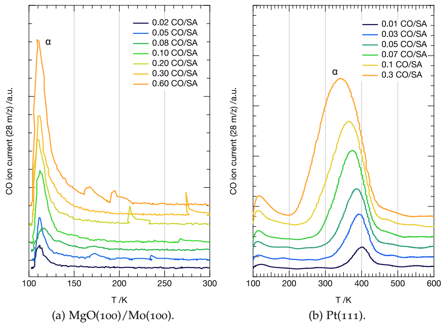
Figure 4.3.1: TPD ( \beta = 2\text{K/s} ) spectra of CO desorption on MgO(100)/Mo(100) (a) and Pt(111) (b). For MgO peak \alpha is assigned to desorption of physisorbed CO. In the case of Pt(111) peak \alpha is attributed to chemisorbed CO.
