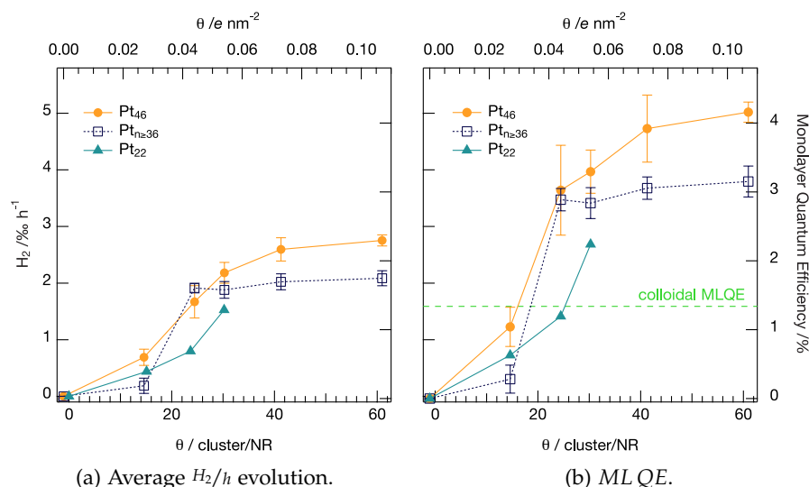
Figure 5.4.6: H_2 production per hour (after four hours of illumination) (a) and MLQE (b) for unselected Pt_{n \geq 36} , selected Pt_{22} and Pt_{46} decorated photo catalysts as a function of cluster coverage. The data points represent the averaged multiple measurements, as shown in fig. 5.4.5b; error bars are based on the standard deviation of these multiple measurements per coverage. The lines connecting the data points serve as a guide to the eye. The maximum performance of the unselected samples is slightly less than for the Pt_{46} samples and saturation sets in at lower coverages. Hydrogen production over Pt_{22} is lower compared to Pt_{46} decorated CdS NRs at similar coverage. In the investigated coverage regime hydrogen yields and MLQE s show qualitatively the same trend with increasing cluster coverage. Corresponding saturation MLQE s of all sample series are higher compared to a colloidal Pt/CdS NRs (green dashed line) photocatalyst system. Reprinted (adapted) with permission from [220] - Copyright (2012) American Chemical Society.
