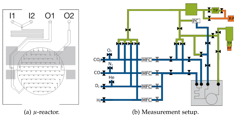
Figure 3.3.5: CAD drawing of a (2 nd gen.) \mu -reactor including the Pt heating structure (gray areas) [96, 309] (a). Gas is introduced from the two inlets (I1,I2), which are connected to the mixing zone. The main flow exits through the main outlet (O1), whereas the products leave the reactor through the capillary outlet (O2) and are fed into a QMS for analysis. \mu -reactor measurement setup at CINP (b). The reactor (grey) is connected via its outlets to a gas manifold system including, manual (black) and pneumatic (grey) valves, mass flow controller (MFC), turbo pumps (TP) as well as rotary pumps (RP) [96, 309]. The different pressure ranges are indicated by the colors: ambient pressure (blue), pre vacuum (orange) and high vacuum (green).
