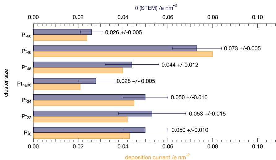
Figure 5.1.2: Statistical analysis of the coverage control of Pt_{n,x} . Discharge current during deposition as comparison (orange), counts from TEM (blue). A minimum of five micrographs per size and for different coverages are taken for the counts. The indicated error for the counted particles is based on the standard deviation of the counts of the individual micrographs.
