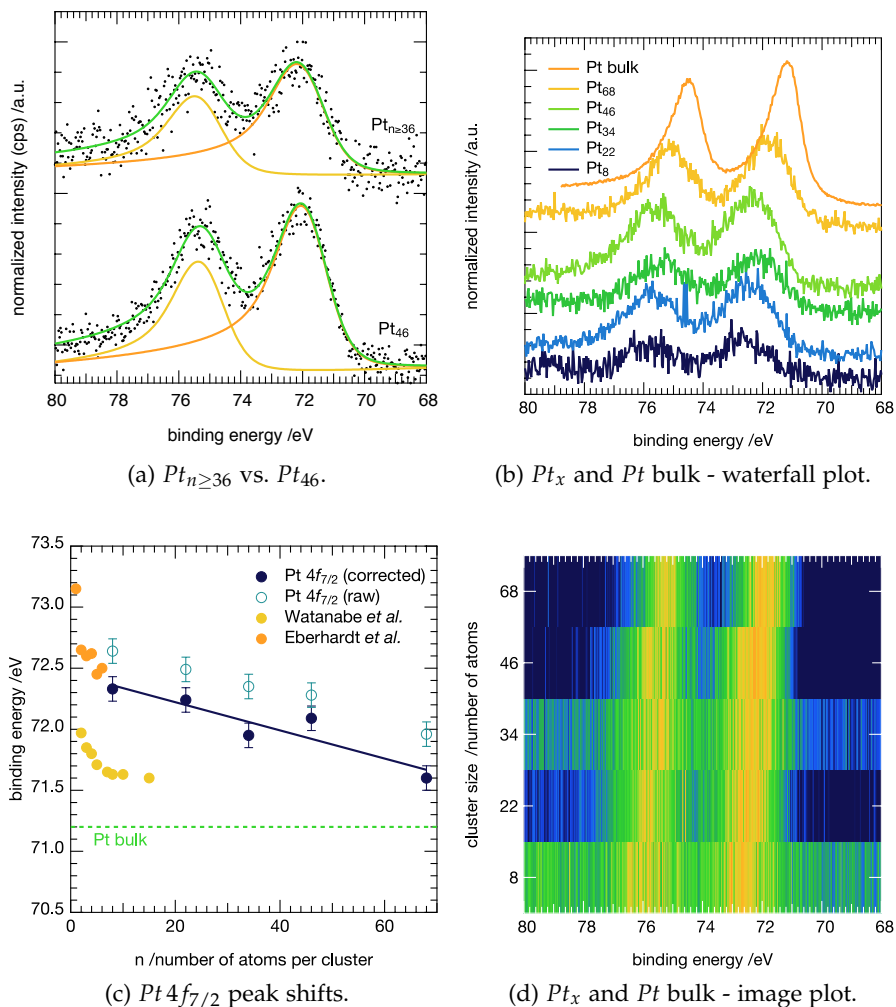
Figure 5.1.11: XPS of Pt 4f peaks for different sizes and comparison to literature values. XPS Pt 4f signals for selected and unselected clusters (a) incl. the corresponding line fit. The normalized Pt 4f signals for different selected cluster sizes and Pt bulk as waterfall plot (b); different sizes as image plot (d). The BE values of the Pt 4f_{7/2} signals as a function of cluster size (c), for comparison the bulk value and BE from measurements in the literature are included.
