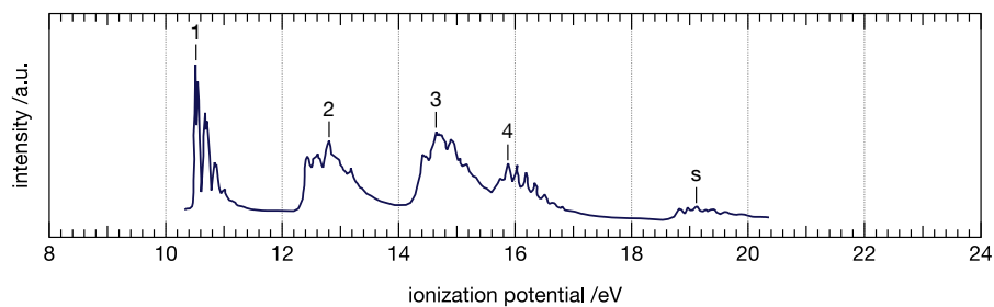
Figure A.3.4: Gas phase photo electron spectrum of ethene adapted from [143].
