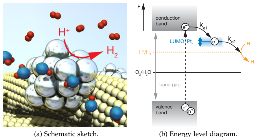
Figure 5.4.9: Size dependent water splitting reaction - schematic sketch of the H^+/H_2 partial reaction (a), energy levels involved in the splitting reaction (b).
