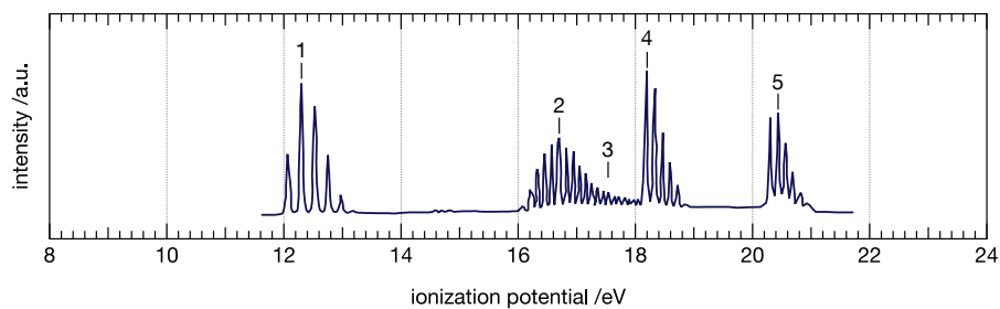
Figure A.3.2: Gas phase photo electron spectrum of molecular oxygen adapted from [143].
