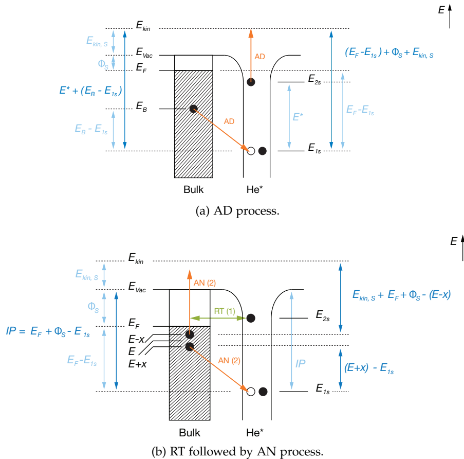
Figure 3.2.6: Underlying MIES processes; AD for metals (a) and RT followed by AN for insulators (b) [213].
