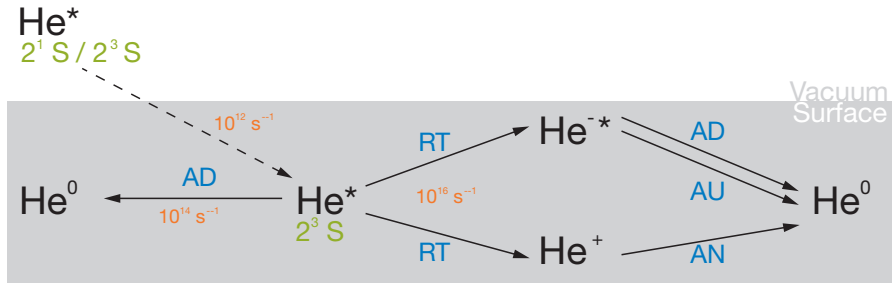
Figure 3.2.5: Reaction scheme describing the possible interactions of a metastable \text{He}^* atom with the surface [213].
