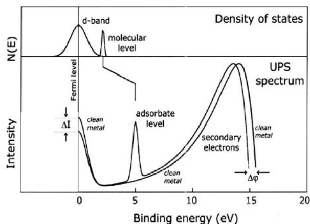
Figure 2.2.1: Schematic UPS spectra of adsorbed species on a d -metal and the corresponding DOS of the metal and MOs of the adsorbed species [41].
