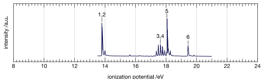
Figure A.3.3: Gas phase photo electron spectrum of carbon dioxide adapted from [143].
