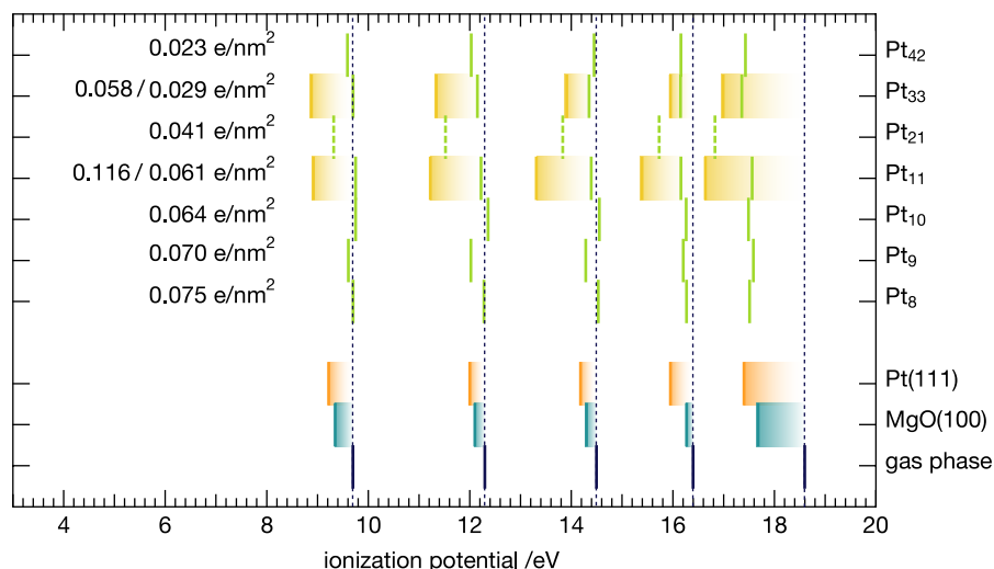
Figure 4.4.15: Shifts of the peak energy positions in MIES of the adsorbed 0.1 TCE/SA TCE on the various cluster sizes with respect to the peak positions of the gas phase spectra of Kimura et al. [143]. As comparison the shifts for an equal amount of TCE adsorbed on the MgO (blue) and the Pt (orange) single crystal surfaces (sec. 4.4.1). Green bars represent low cluster coverage; for Pt_{11} and Pt_{33} additionally a higher coverage was probed (yellow).
