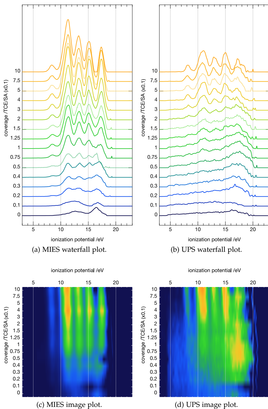
Figure 4.4.5: EE spectra (MIES a and UPS b) of adsorbed TCE on Mo(100); referenced against the vacuum level and background corrected. Increasing dosage of TCE from bottom to top; MIES (a) and UPS (b). The bottom spectra show the clean Mo(100) surface. The dashed lines indicate the coverages (0.05, 0.15 and 0.5 TCE/SA) for which the IP peak energy shifts are shown in fig. 4.4.10; with 0.15 TCE/SA corresponding to data from a completed first monolayer (dashed line). Subfigures (c) and (d) show the corresponding image plots for better visibility of the appearance of the TCE peak features for MIES and UPS, respectively. Reprinted (adapted) with permission from [172] - Copyright (2012) Elsevier.
