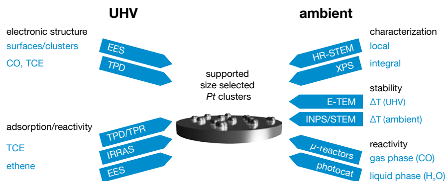
Figure 1.3.1: Schematic sketch of the thesis approach to further the understanding of Pt cluster catalyst materials under UHV (left) and ambient (right) conditions. The main focus points are depicted in black, the studied systems/aims in blue and the techniques with the arrows.
