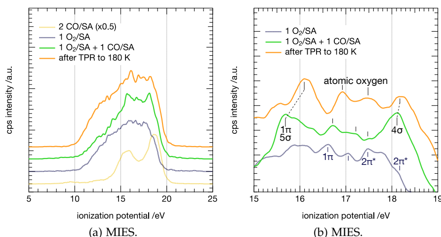
Figure 4.3.5: MIE spectra with 1 O_2/SA , 2 CO/SA as well as 1 O_2/SA with 1 CO/SA before and after TPR reaction to 180 K on Pt(111). Overview spectra (a) including the CO spectra from the previous section for comparison; in excerpt (b) the spectral features are assigned to MOs, for details see text.
