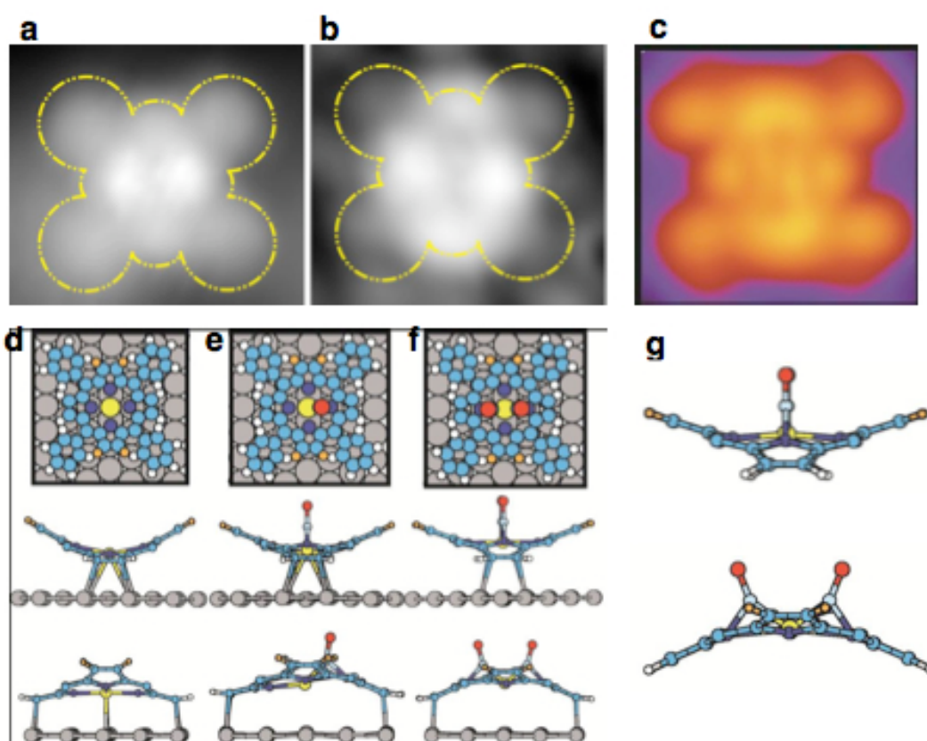
Figure 3 Comparison of experimental data and theoretical description. STM images of a (\text{CO})_2/\text{Fe-TPP} on \text{Ag}(111) and b (\text{CO})_2/\text{Co-TPP} on \text{Cu}(111) c The image simulation for (\text{CO})_2/\text{Co-TPP} with two \mu -carbonyl adducts on \text{Cu}(111) from DFT reproduces the main features of the experimental STM data. d-f DFT modeling showing the relaxed geometry of the systems \text{Co-TPP} ( d ), \text{CO/Co-TPP} ( e ) and (\text{CO})_2/\text{Co-TPP} ( f ) on \text{Cu}(111) with bridging \mu\text{CO} ligation. g DFT model of stable, free (\text{CO})_2/\text{Co-TPP} species in cis- \mu -dicarbonyl geometry.
