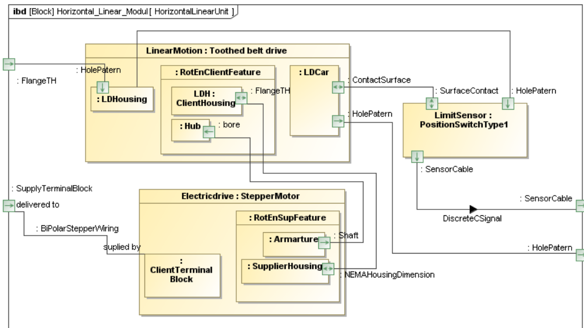
Figure 47: Internal block diagram showing specific components of a horizontal linear motion unit
