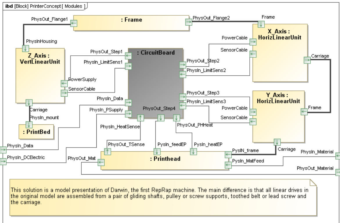
Figure 48: Product level structure of the whole printer
